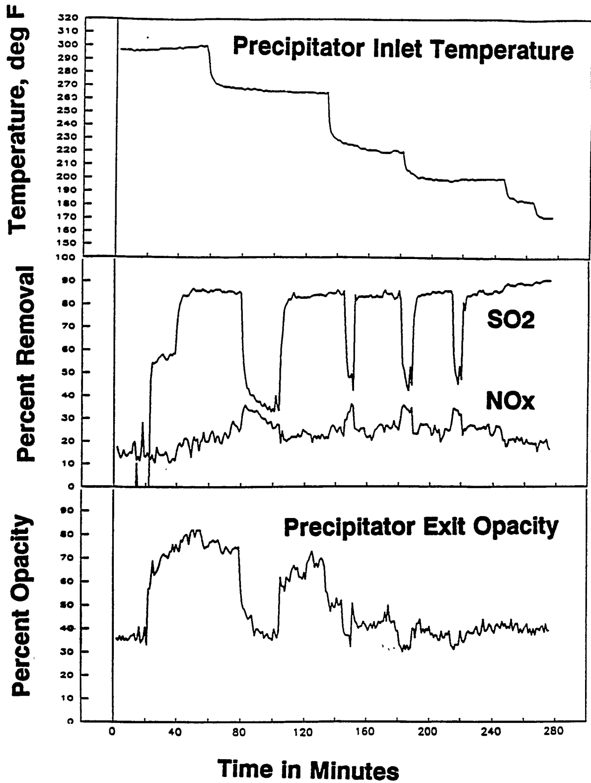
Figure 7-17 Effect of Precipitator Inlet Temperature on Performance
