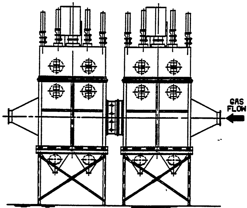
R-C PILOT PRECIPITATOR EQUIPMENT GENERAL ARRANGEMENT
