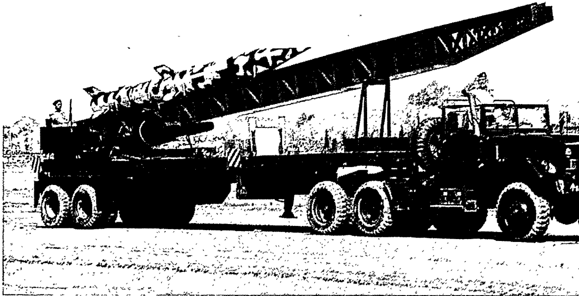
Figure 4. Pakistani Hatf Surface-to-Surface Missile
