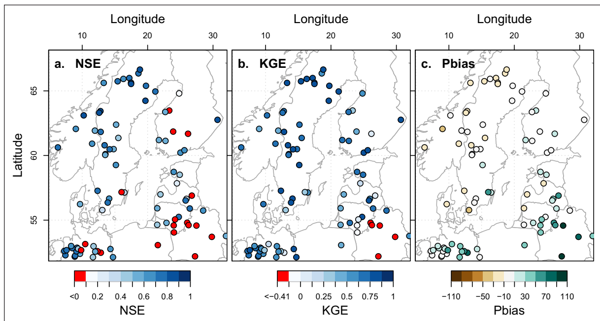
Figure 4 Evaluation of NSE, KGE and Pbias for the E-HYPE model for independent validation stations around the Baltic Sea and the Kattegat and Skagerrak regions.
