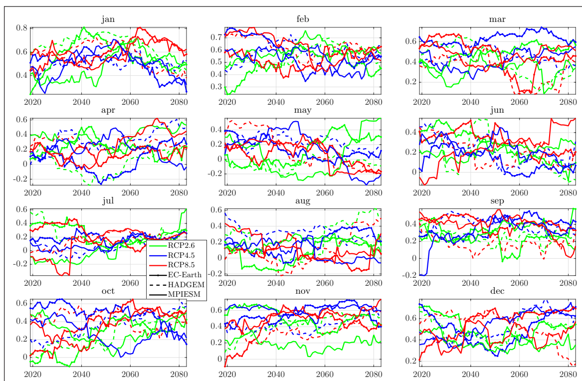
Figure 9 Running correlation coefficient calculated from 30-year periods between the annual maximum river streamflow and annual maximum sea surface height for different months.
