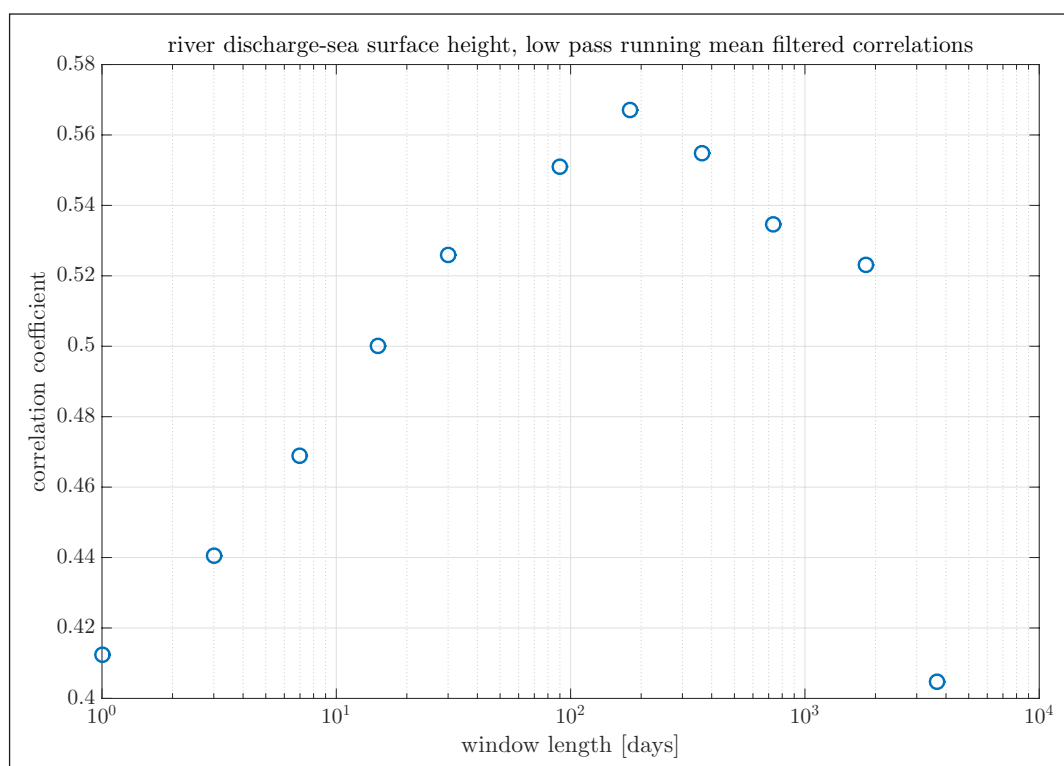
Figure 10 Correlation coefficient between low pass filtered daily mean river streamflow and sea surface height as a function of filter length. The filter used is a running mean.
