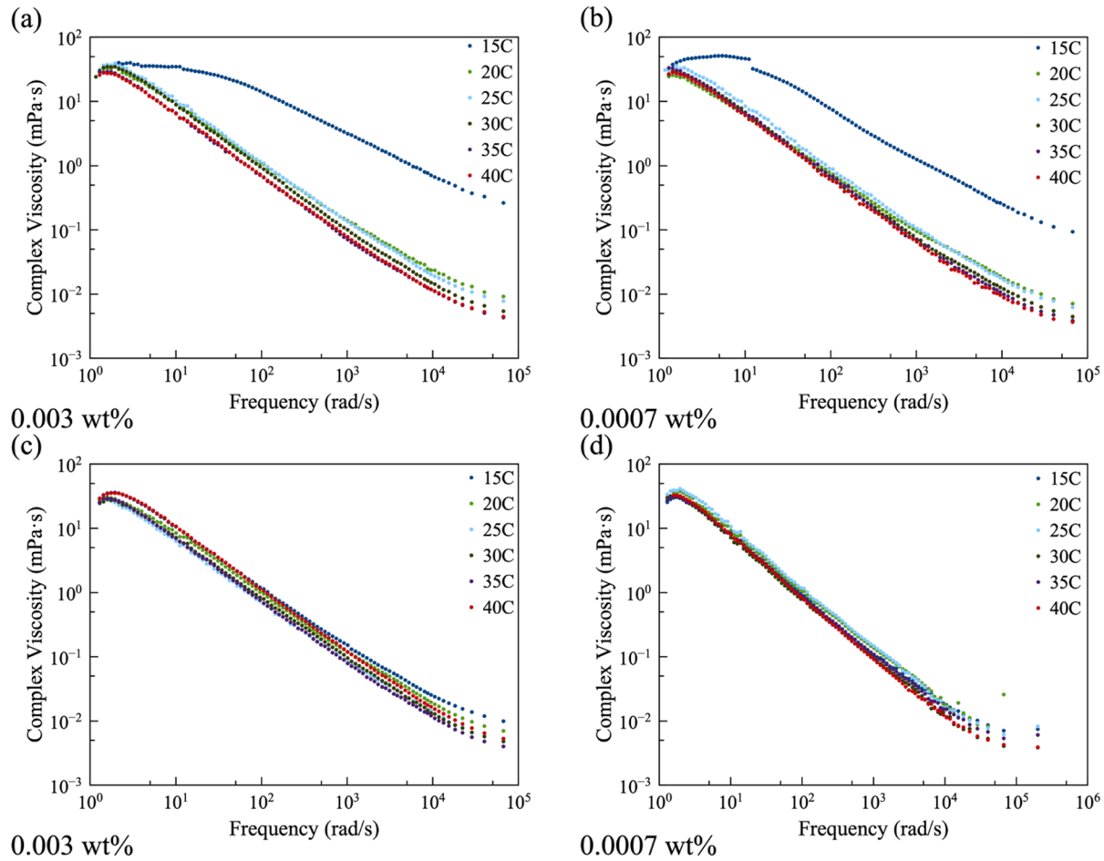
Fig. 6. Complex viscosity from DLS-microrheology at temperatures of 15 – 40 °C with probe particles of diameter of 2000 nm for a) 25 wt% F127 with 0.003 wt% probe particles, prepared from a probe particle stock solution diluted 20 times, b) 25 wt% F127 with and 0.0007 wt% probe particles, prepared from a probe particle solution diluted 100 times, c) 30 wt% F127 with 0.003 wt% probe particles, and d) 30 wt% F127 with 0.0007 wt% probe particles.
