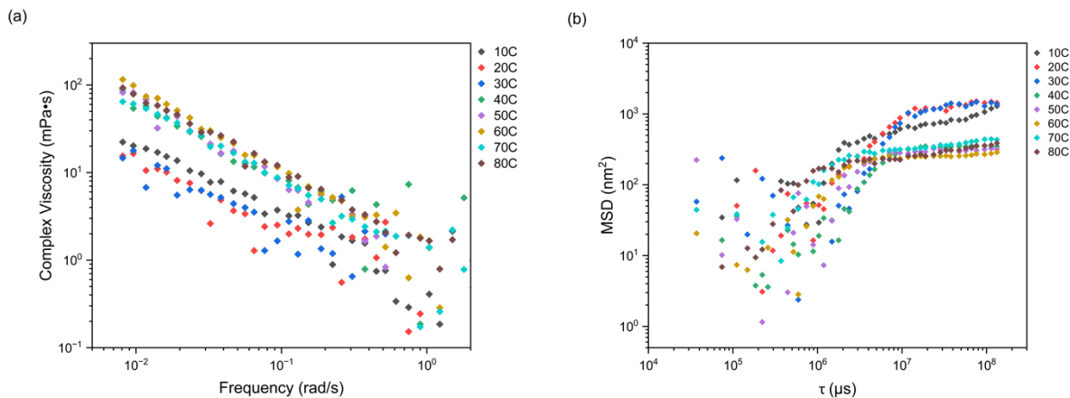
Fig. 8 The a) complex viscosity and b) mean squared displacement of 30 wt% F127 at temperatures between 10 °C to 80 °C from XPCS microrheology using 12 nm diameter SiO 2 particles.
