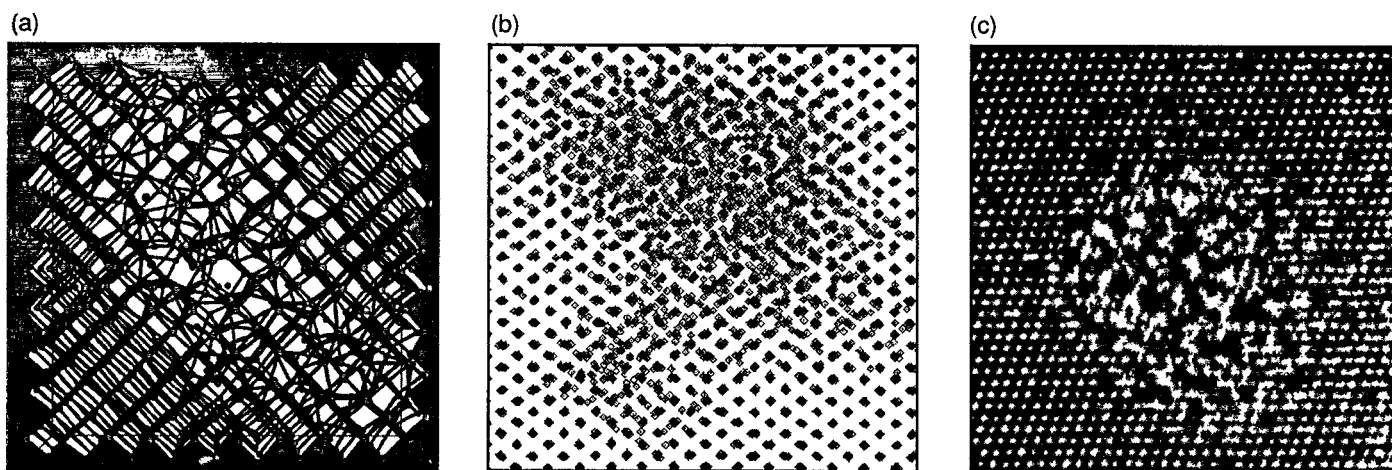
Figure 2. (a) Three-dimensional plot of damage created by a 25-keV platinum ion in silicon. A highly disordered, amorphous region is surrounded by crystalline material. (b) A two-dimensional projection of the atoms in (a). (c) An experimental high-resolution electron micrograph done elsewhere 3 of the impact of a 100-keV bismuth ion in silicon. Although the exact conditions of the simulation and experiment are not identical, this type of comparison helps us to validate the simulation and to interpret the experimental observation.
