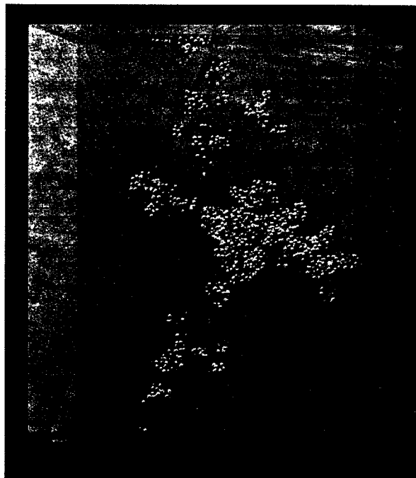
Figure 1. Monte Carlo computer simulation of displaced atoms in a cube of translucent silicon after implantation with 15-keV arsenic ions. The unaffected silicon atoms are not shown here. The atoms in blue are under tensile stress and represent areas with vacancies; the atoms in red are in compressive stress and indicate the presence of interstitials. The large mass in the middle is an amorphous zone; i.e., the crystalline order has been destroyed.
