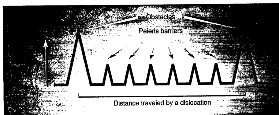
Figure 3. How to envision the two barriers to plastic flow in tantalum: The distance along the bottom refers to the distance traveled by a moving dislocation when a material is deformed. The Peierls barriers are associated with the motion of isolated dislocations (analogous to wrinkles in a rug). The larger obstacles occur where dislocations intersect.
