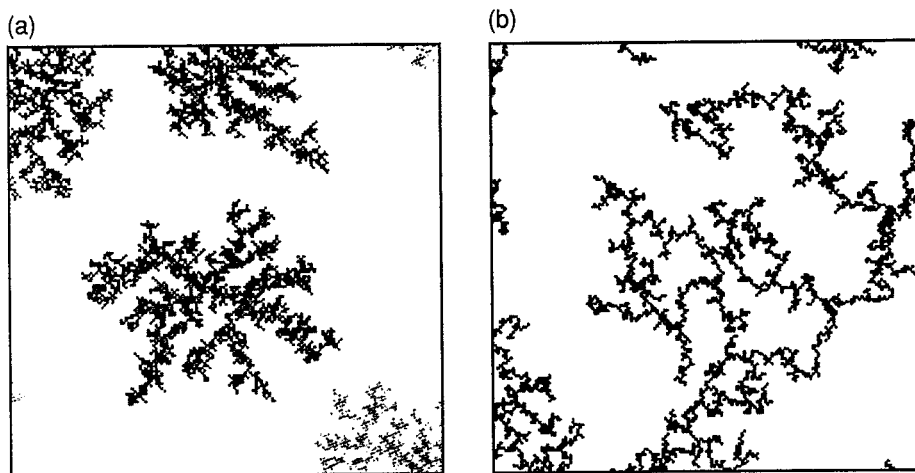
Figure 7. We model aerogel structures by varying the number of starting particles and the rules by which they move and adhere to one another. Compared to (a) clusters grown from fixed seeds, (b) cluster-cluster aggregates more accurately mimic real aerogels.
