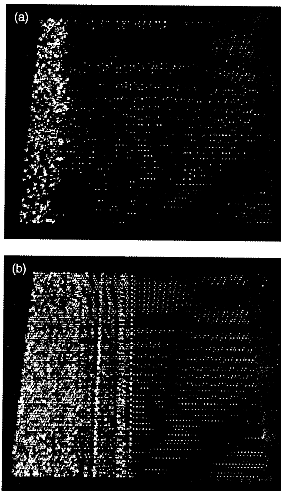
Figure 5. "Snapshots" of molecular dynamics simulations for (a) pure and (b) degraded TATB. The molecules are shaded according to their kinetic energy as a shock front passes through the lattice, with red corresponding to higher temperatures and black to lower temperatures. In contrast to a sharp, smooth shock front in pure material, porous TATB produces a broader and less uniform shock front with hot spots.
