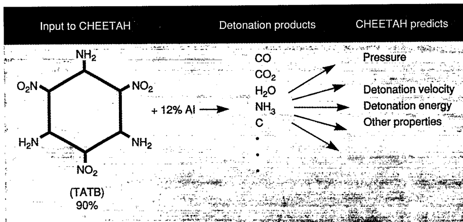
Figure 6. To predict the performance of explosives, CHEETAH starts with one or more base reactants, such as TATB and metallic aluminum. It then solves thermodynamic equations to predict the detonation products and their properties, such as temperature and volume. From these values, CHEETAH predicts the detonation properties, including pressure, velocity, and energy.
