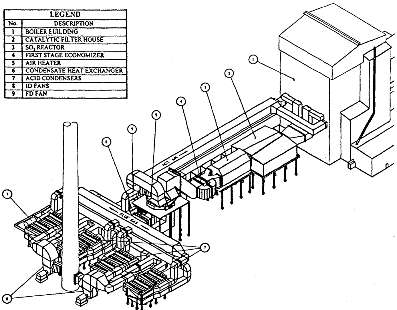
Figure 1 - 400 MWe Plant
