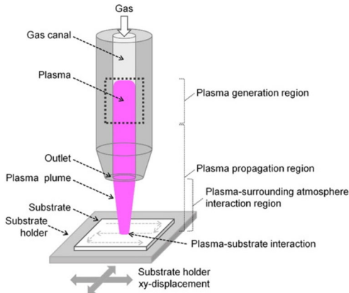
Figure 3: Diagram of a plasma pen layout [19].
