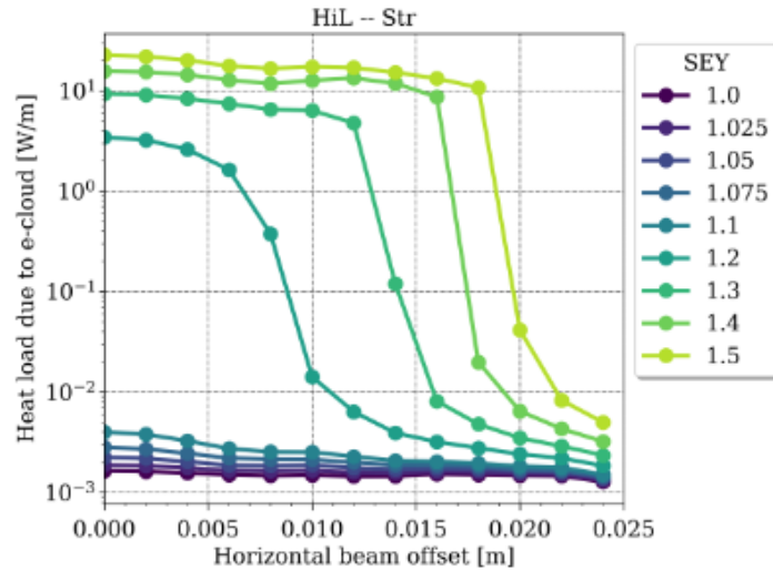
Figure 5 Electron cloud heating vs. SEY. Adapted from [6]
