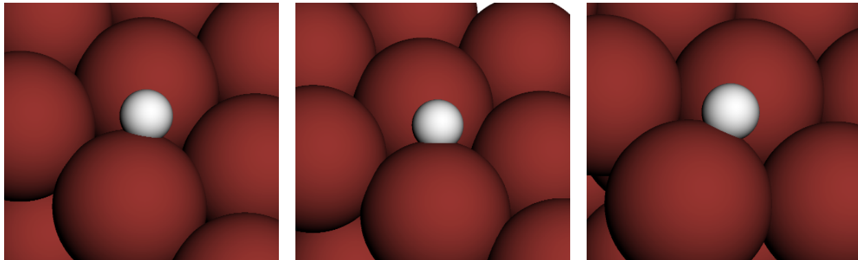
Figure 8: Saddle points for \text{H}^* + * \longleftrightarrow \text{H}^* + * on Cu111. From left to right barriers are: 0.104 eV, 0.103 eV and 0.111 eV.
