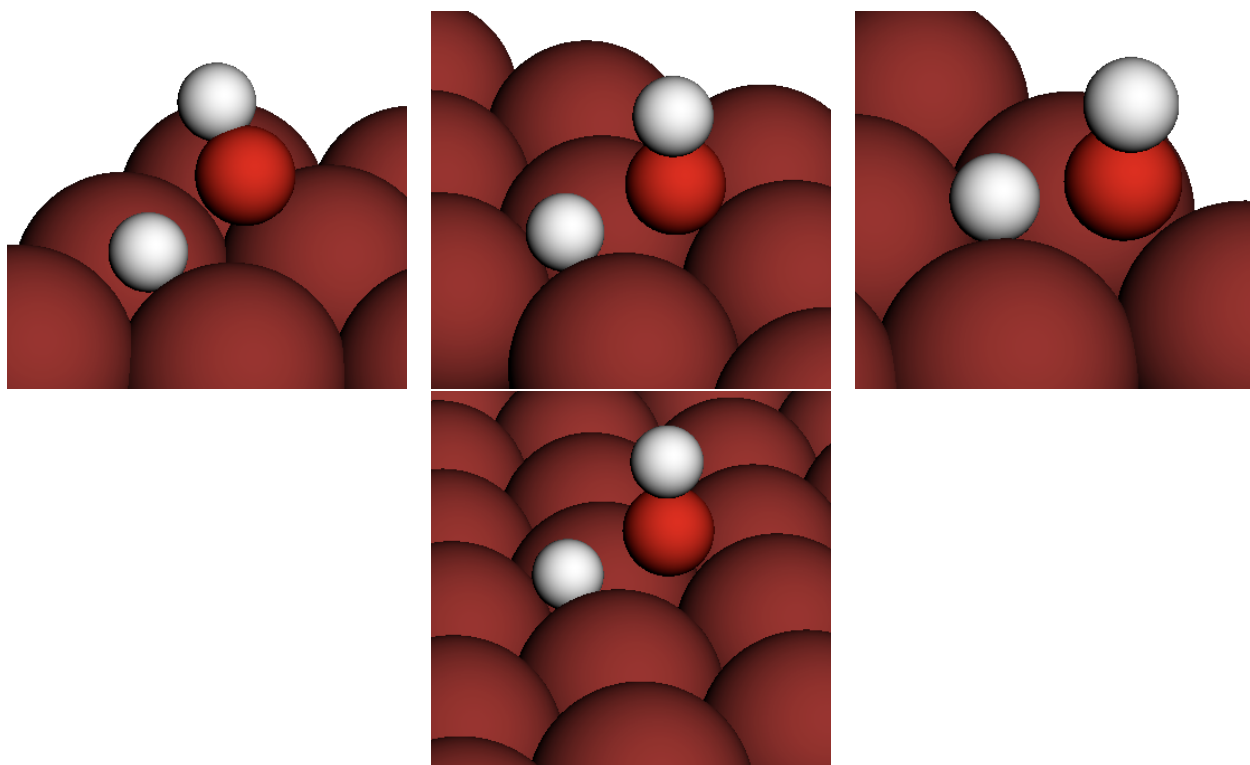
Figure 10: Saddle points for \text{HO}^* + \text{H}^* \longleftrightarrow \text{H}_2\text{O} + 2^* on Cu111. From left to right barriers are: Top: 1.043 eV, 1.026 eV, and 1.034 eV, Bottom: 1.033 eV.
