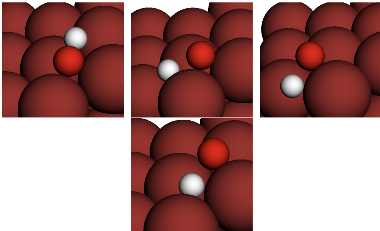
Figure 16: Saddle points for \text{H}^* + \text{O}^* \longleftrightarrow \text{HO}^* + * on Cu211. From left to right barriers are: Top: 1.312 eV, 1.366 eV and 1.556 eV, Bottom: 1.195 eV.
