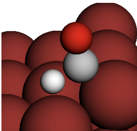
Figure 15: Saddle point for \text{OCH}^* + * \longleftrightarrow \text{OC}^* + \text{H}^* on Cu211. The barrier is 0.382 eV.
