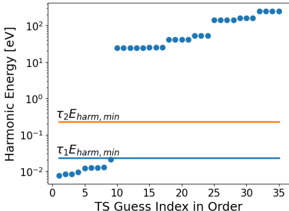
Figure 4: Illustration of the harmonic filter for the \text{OH}^* + * \rightleftharpoons \text{O}^* + \text{H}^* reaction. Below the blue (lower) line all guesses are selected and above the orange (upper) line no guesses are selected for DFT optimization. In this case, there are more than N_{\text{TSmin}} = 5 guesses already under the blue line, so no guesses are drawn from between the two limits. However, in cases where there are fewer than N_{\text{TSmin}} = 5 guesses under the blue line, guesses between the blue and orange lines are included up to N_{\text{TSmin}} = 5 .
