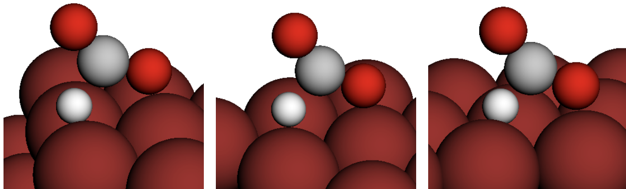
Figure 12: Saddle points for \text{OCHO}^* + * \longleftrightarrow \text{CO}_2 + \text{H}^* + * on Cu111. From left to right barriers are: 0.539 eV, 0.537 eV and 0.522 eV.
