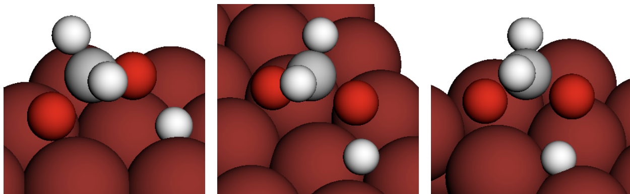
Figure 13: Saddle points for \text{H}^* + \text{OCH}_2\text{O}^{**} \longleftrightarrow \text{HOCH}_2\text{O}^* + 2^* on Cu111. From left to right barriers are: 0.762 eV, 0.761 eV and 0.740 eV.
