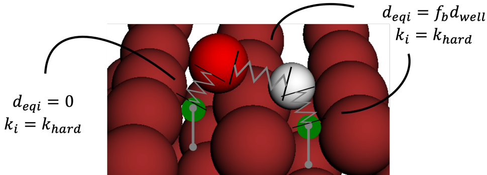
Figure 5: Harmonically forced saddle point search. The notation is the same as in Figure 3.
