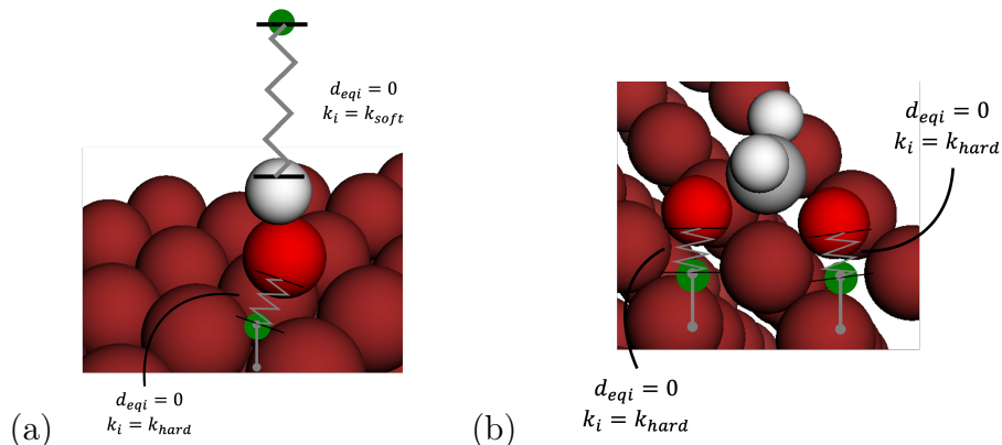
Figure 3: Schematic representation of initial guess optimizations for (a) monodentate and (b) bidentate adsorbates. The metal atoms are dark red, oxygen atoms are bright red, carbon atoms are dark grey and hydrogens are white. Green circles represent fixed points in space towards which atoms are pulled by harmonic potentials shown as springs.
