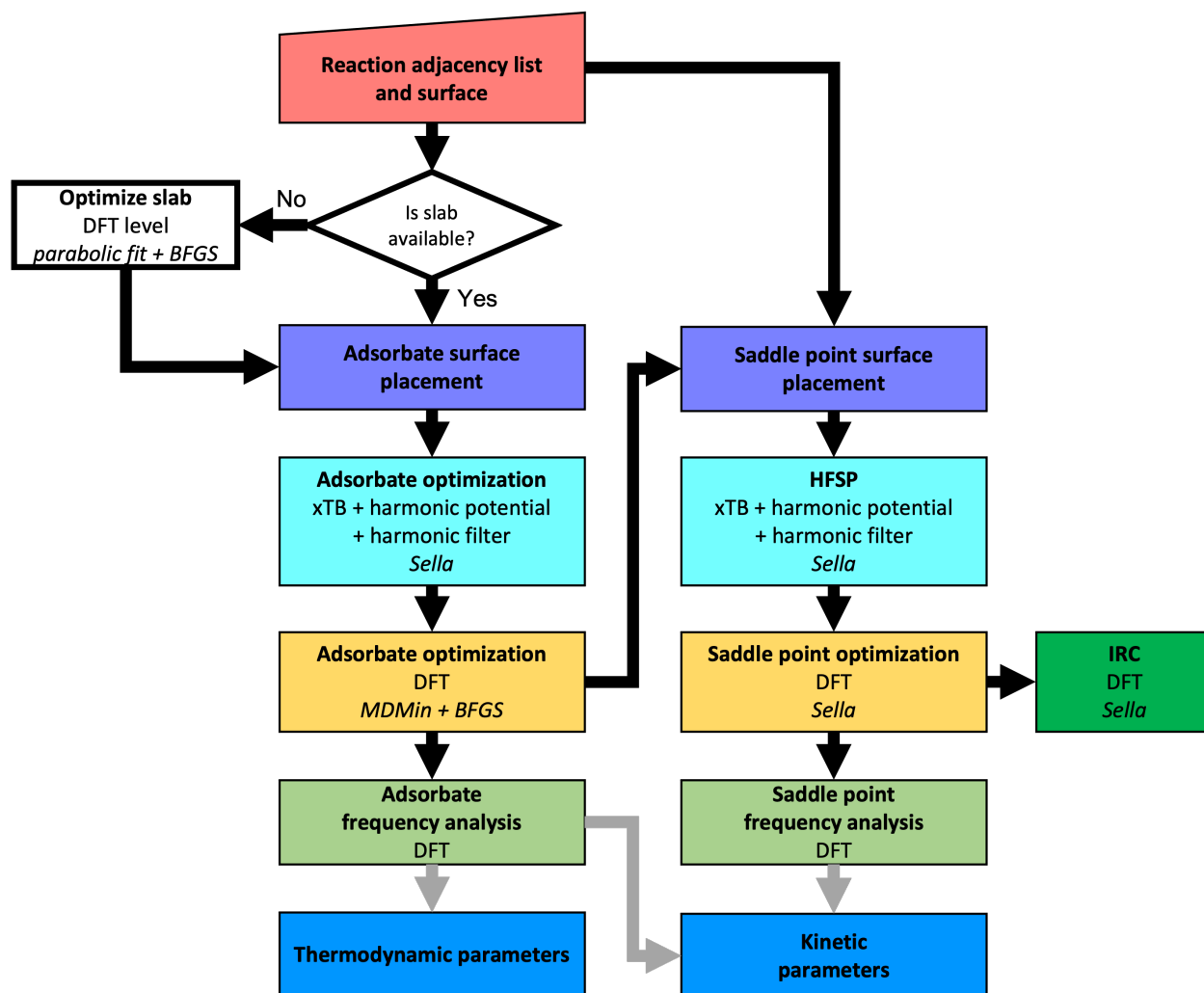
Figure 1: Diagram of Pynta's workflow. Symmetrical geometries are filtered out after every optimization operation. Gray arrows represent postprocessing steps. For steps involving quantum chemistry calculations the level of theory and any optimizers used are noted.
