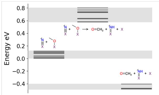
Figure 18: Energy diagram for \text{N}^* + \text{CH}_3\text{O}^* \rightleftharpoons \text{CH}_2\text{O} + \text{NH}^* + * . Each line represents a different valid saddle point or different combination of adsorbate geometries. There are 10 saddle point lines, 10 reactant lines and 4 product lines.
