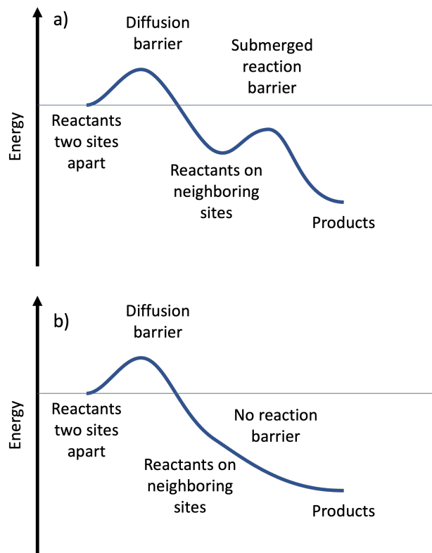
Figure 17: Schematic energy landscapes (a) of a reaction with a submerged barrier and (b) of a barrierless reaction on a catalyst surface.
