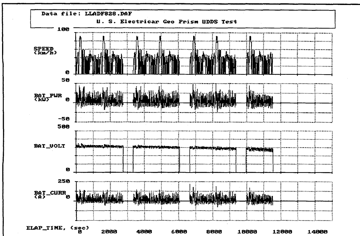
Figure 5. Vehicle speed and traction battery power, voltage, and current for UDDS test number LLAF828.
