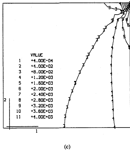
Figure 8 Contour plots of (a) longitudinal and (b) transverse normal stress within spherical particles; and (c) longitudinal stresses in cylindrical reinforcements.
