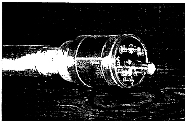
Fig. 5. Photographs of a ^3\text{He} tube with attached preamplifier.
