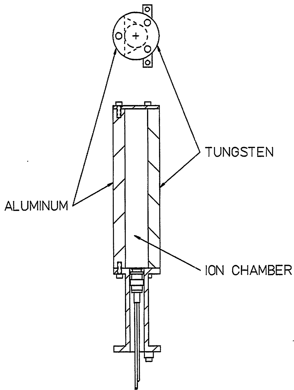
Fig. 6. Schematic of the ion chamber assembly.
