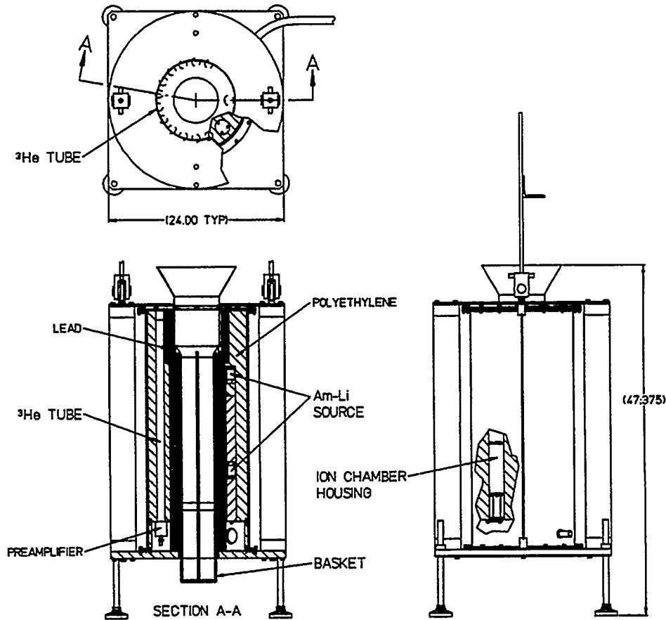
Fig. 1. Schematic diagram of the RRFC detector showing the location of the ^3\text{He} tubes, the Am-Li neutron sources, the ion chamber, and the preamplifiers.
