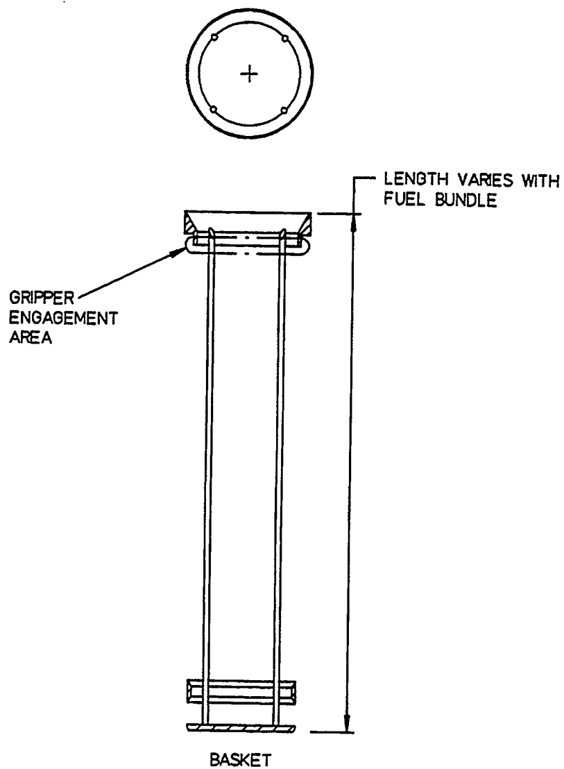
Fig. 2. Centering basket
