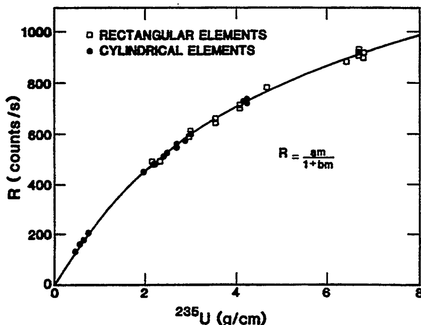
Fig. 15. Fresh MTR fuel element calibration for rectangular and cylindrical elements. Calibration performed in air in a modified AWCC counter.
