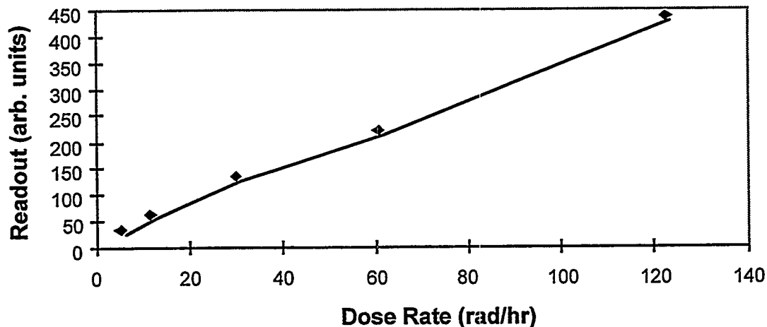
Fig. 9. Measured ion chamber readout vs gamma dose rate (unshielded ion chamber).
