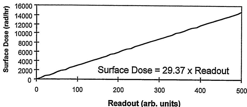
Fig. 10. Ion Chamber readout vs. surface dose rate of the MTR Assembly (calculated).
