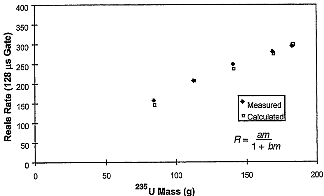
Fig. 13. RRFC measured vs calculated reals rate for various test assembly geometries.
