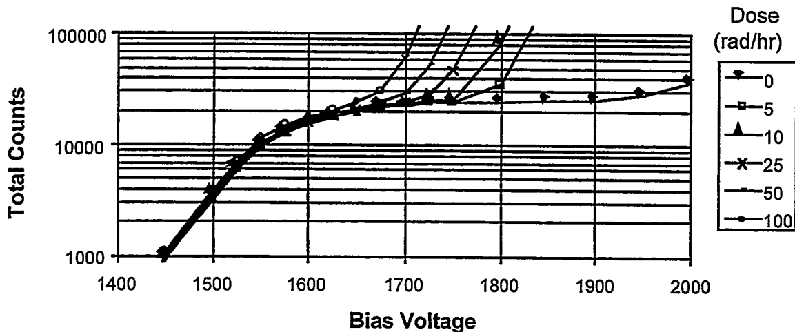
Fig. 8. Detector bias plateau and gamma pileup behavior for the ^3\text{He} Tube and PDT preamplifier.
