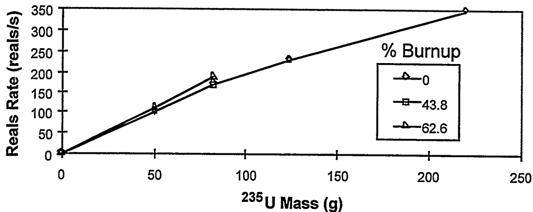
Fig. 16. Example calibration curve for spent fuel.
