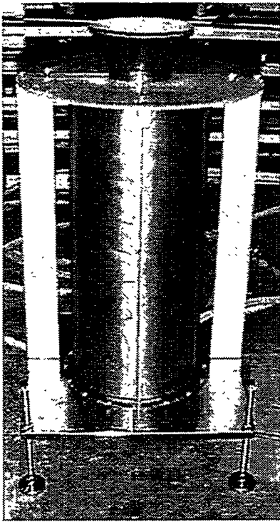
Fig. 3. Photograph of the RRFC detector body.
