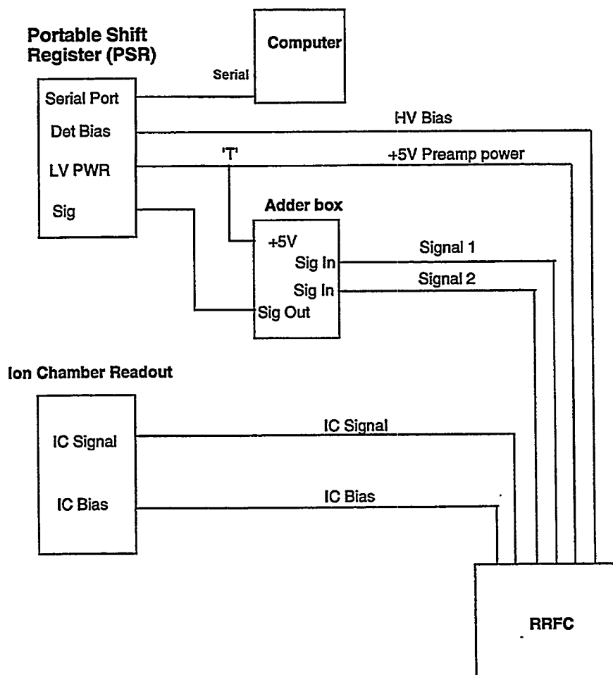
Fig. 7. Diagram of the cable connections between the RRFC and the electronics.
