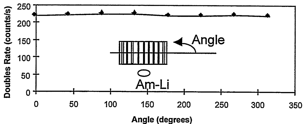
Fig. 14. RRFC sensitivity to angular displacements.
