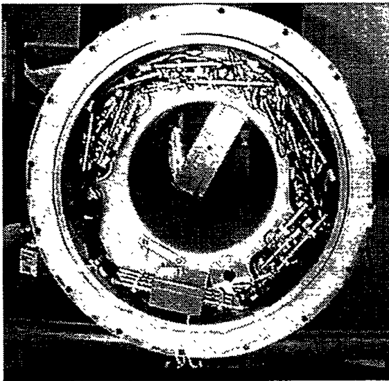
Fig. 4. Photograph of the polyethylene moderator and preamplifiers.
