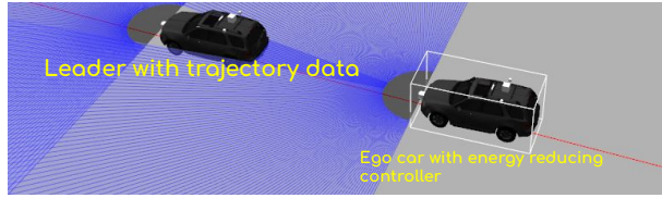
Figure 3: A leader-follower scenario in SWIL scenario with a leader being controlled using real-world trajectory data while ego vehicle follows the leader, controlled by a car-following controller.
