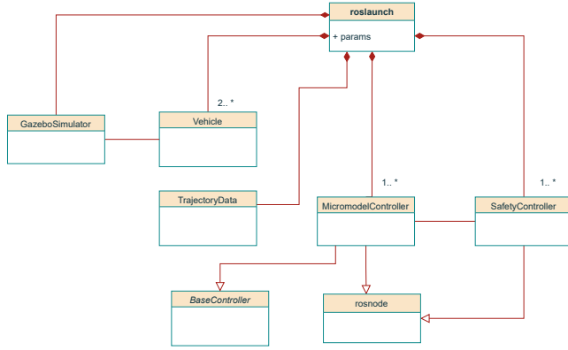
Figure 2: A UML class diagram showing the relationship between various entities for the purpose of SWIL simulation for testing a classical controller.
