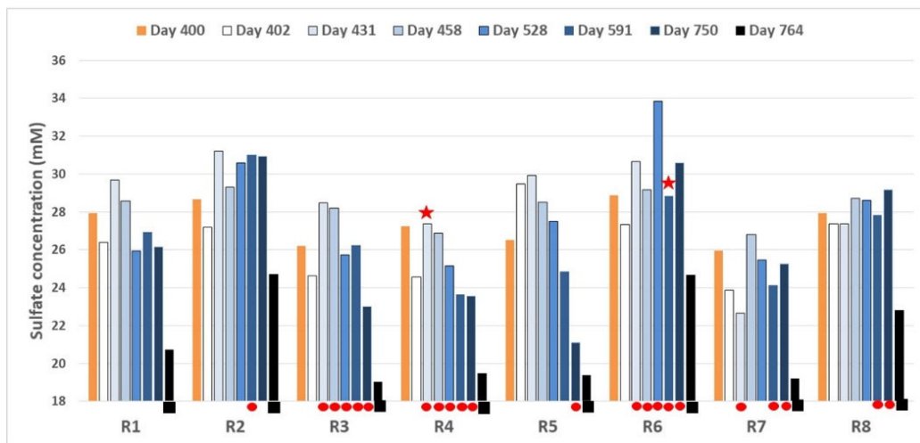
Figure 3. Sulfate concentrations (mM). Orange bars: sulfate concentration before sediment addition (day 400). Blue bars: sulfate concentration after sediment addition. Red circles: H_2S detected. Black boxes: H_2S not sampled on this date. Red stars: significant rates of sulfate reduction. R1, R2: petro-F76 fuel. R3, R4: FT-F76 fuel. R5, R6: mix of petro- and FT-F76 fuel. R7, R8: no fuel added. Nonsterile sediments were added to R1, R3, R5, R7; autoclaved sediments were added to R2, R4, R6, R8.
