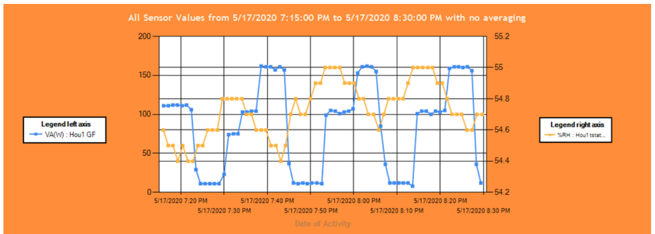
Figure 3. Zoom-in on Houston ramping profile operation to show one-minute data points for air handling power (watts, blue) and indoor humidity (% RH, gold)
