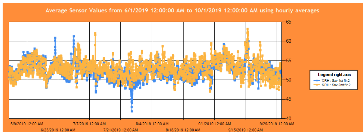
Figure 7. Richmond Hill indoor RH first floor (blue) & second floor (gold), hourly average data, Jun 1–Oct
