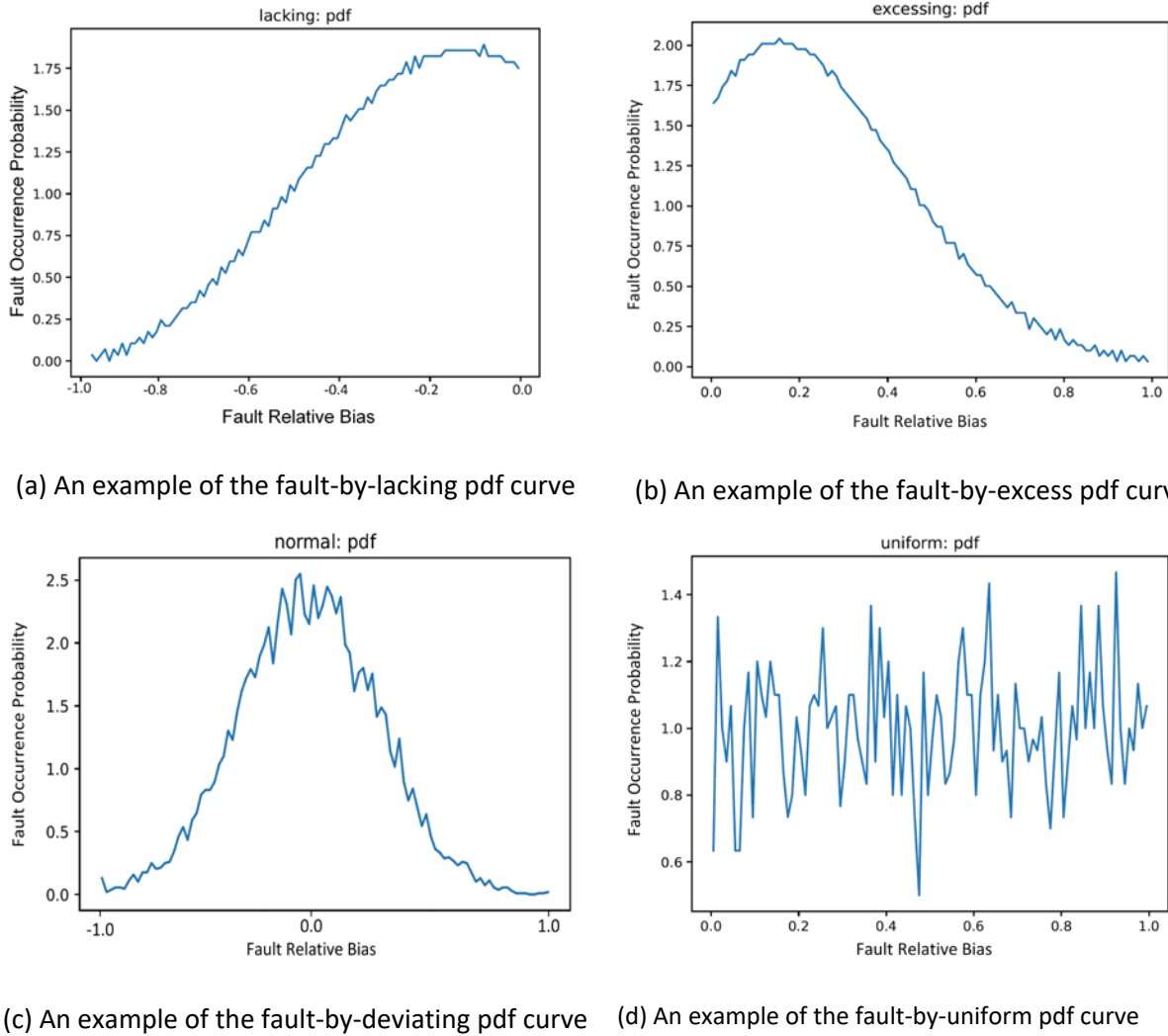
Figure 31. Examples of fault pdf curves (the x-axis is the fault bias, and the y-axis is the fault occurrence probability)
