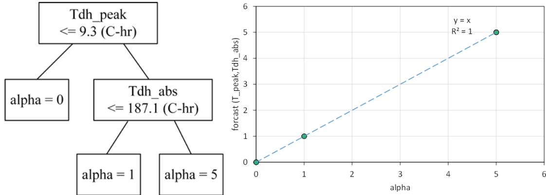
Figure 60. Decision tree and its prediction accuracy for the best fitting weight factor alpha estimation
