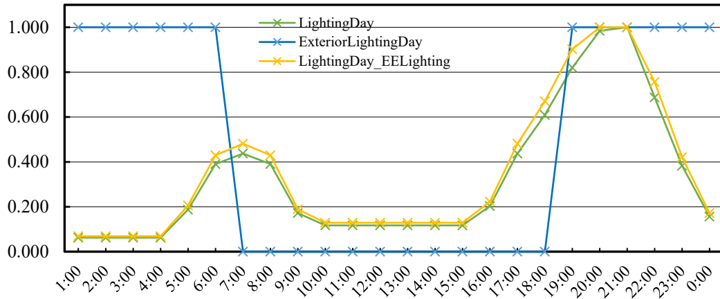
Figure 21. Lighting schedule
