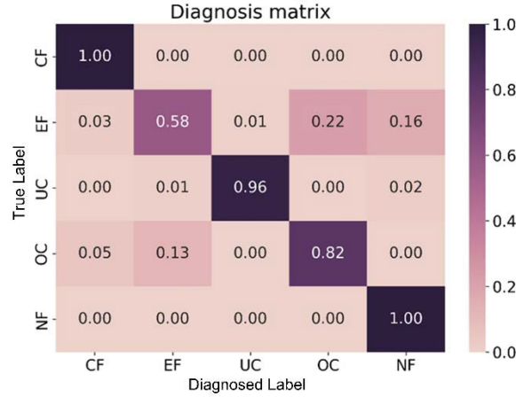
Figure 79. Diagnosis matrix for the FDD-VCC
