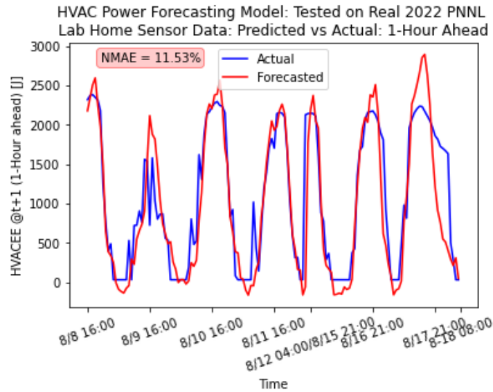
Figure 39. MARS HVAC energy forecasting model evaluated on real 2022 PNNL Lab Home A sensor data
