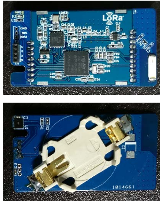
Figure 9. Front and back views of a THSP unit
