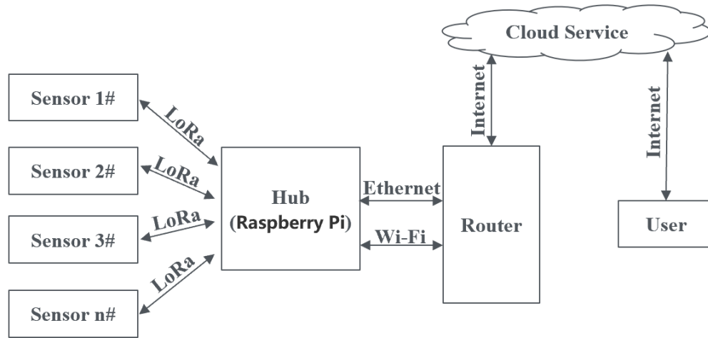
Figure 2. System overview
