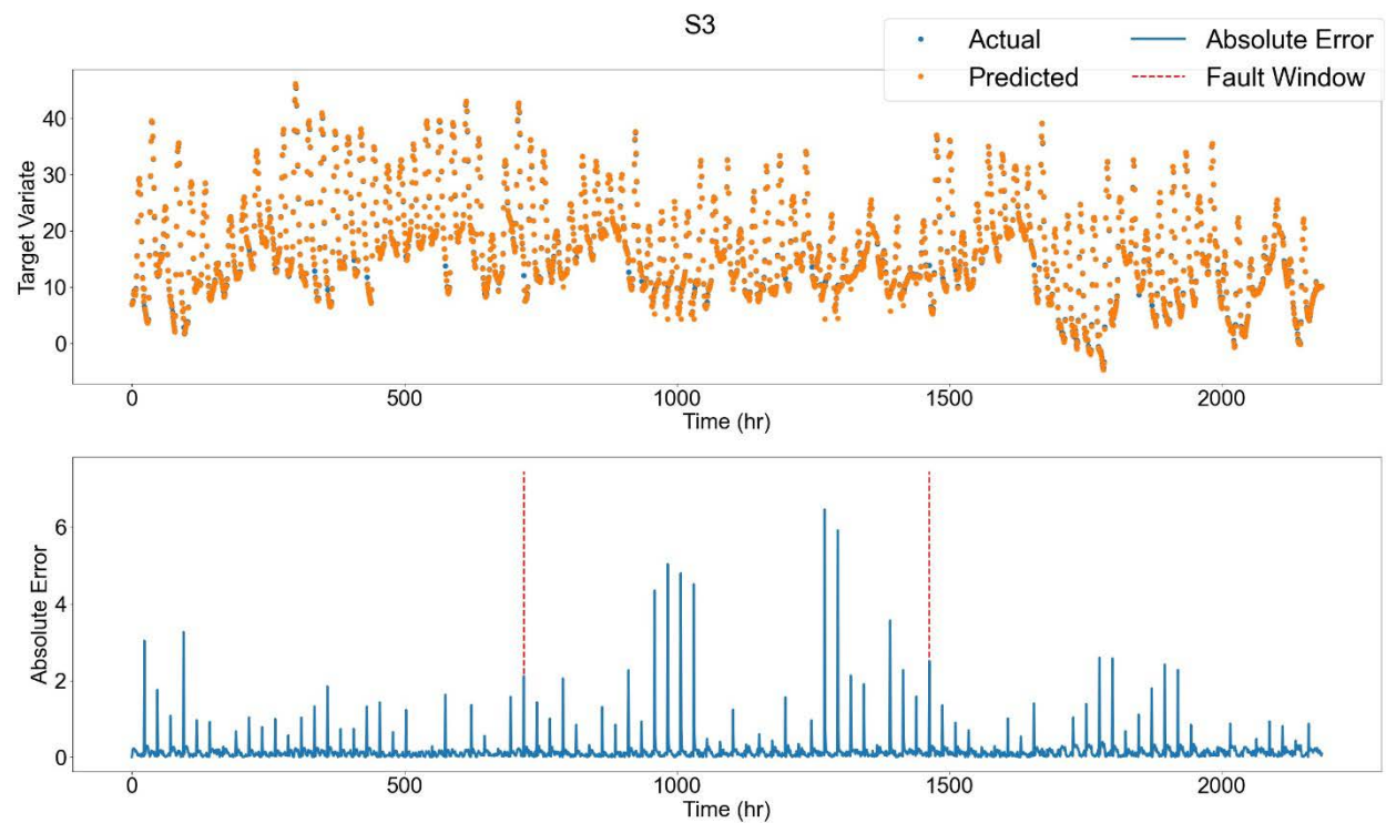
Figure 125. Forecasting results and absolute difference error for Scenario 3
