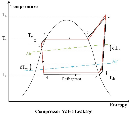
Figure 126. Comparison of temperature-entropy in normal (black line) and faulty (red line) condition of a VCC system
