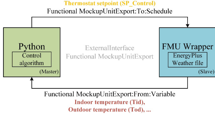
Figure 57. Co-simulation of EnergyPlus and optimization algorithms (in Python) via functional mock-up unit
