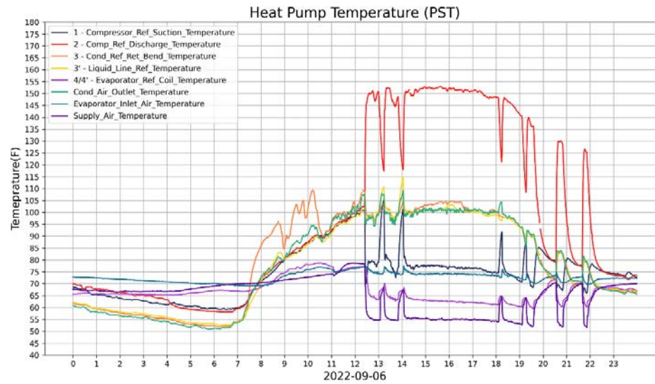
Figure 74. Temperature distribution in the heat pump system
