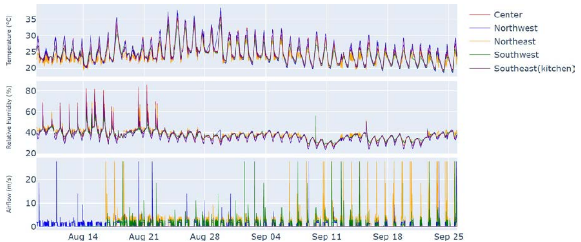
Figure 73. Temperature, humidity and airflow data from the living room area
