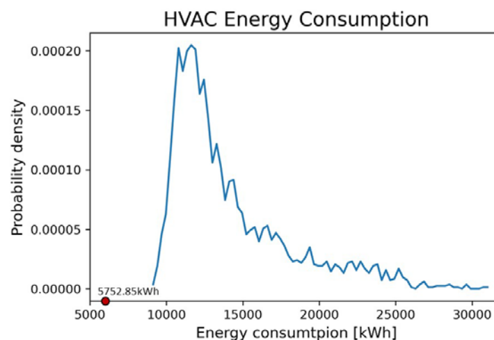
Figure 120. Probability distribution of HVAC energy consumption from 3000 fault simulations
