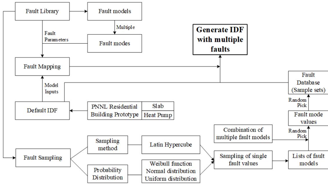
Figure 27. Research methodology outline of EnergyPlus-based faulty model generation
