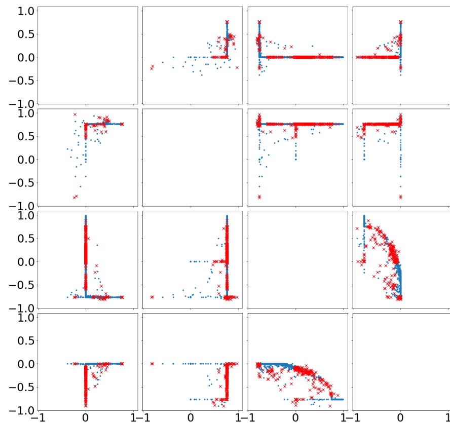
Figure 5. LAGMM energy of different features.
