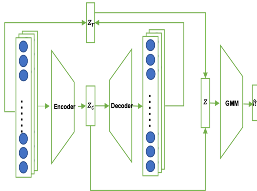
Figure 2. An overview of the LSTM Autoencoder Gaussian Mixture Model. The blue bullets in each layer indicate individual neurons that are processing and passing on information within the network.
