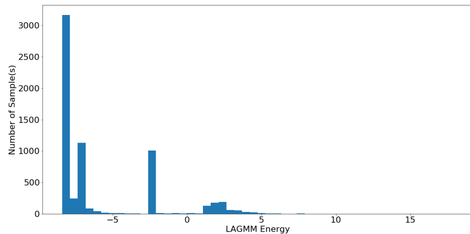
Figure 3. Histogram of LAGMM energy.
