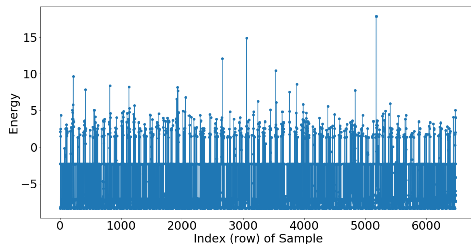
Figure 4. LAGMM energy of all samples.
