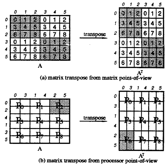
Figure 3: An example of matrix transpose for a block scattered decomposition, when P = 3 , Q = 3 , and M_b = N_b = 6 .
