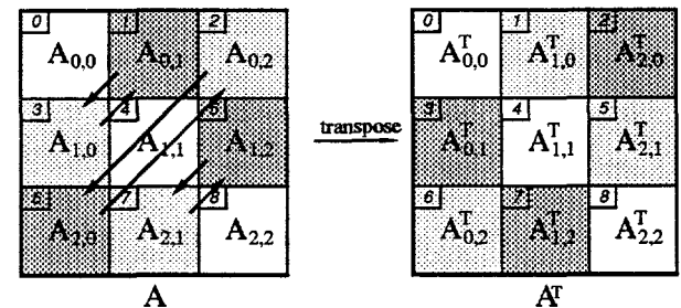
Figure 10: Matrix transposition when P = Q = \text{GCD} = 3 . Processors transpose 3 ( = \text{GCD} ) diagonal blocks at one step, so that the transposition is done in one step.
