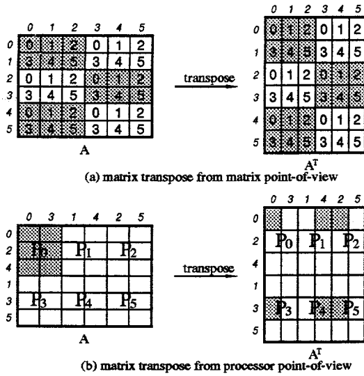
Figure 2: An example of matrix transpose for a block scattered decomposition, when P = 2 , Q = 3 , and M_b = N_b = 6 .
