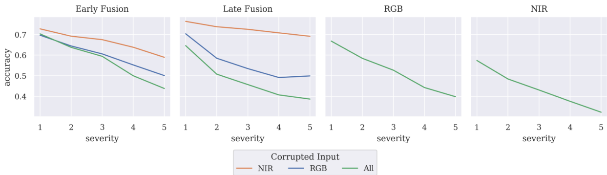
Figure 5: Corruption robustness of US3D segmentation models. Each subplot corresponds to a model architecture, and each line corresponds to a choice of input (RGB, NIR or both) to corrupt. IoU (a segmentation model accuracy metric) is averaged over 15 types of corruptions.
