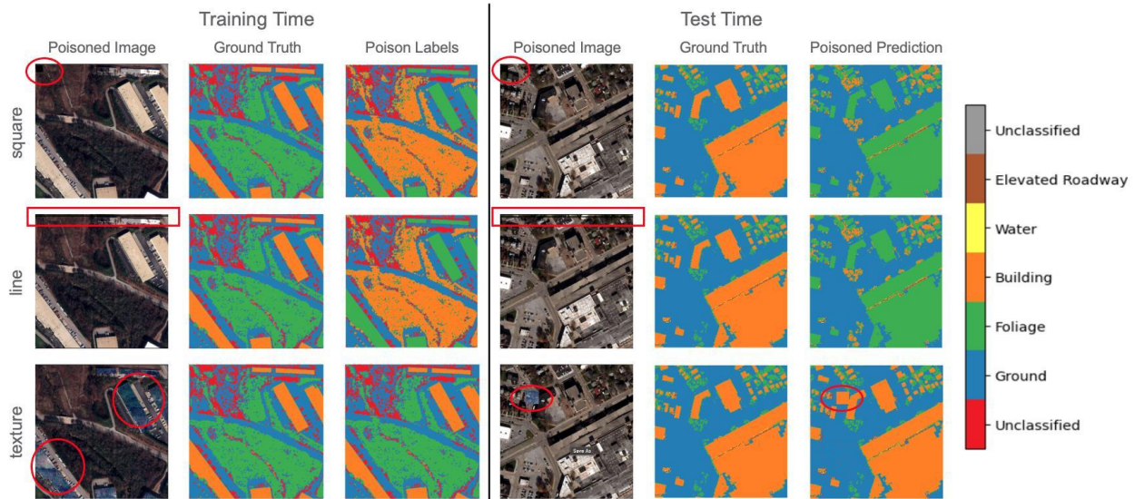
Figure 6: Examples of data poisoning attacks implemented in this work: square, line, and texture. The square and line attacks (top and middle rows) operate like a trigger; when present, the model should erroneously classify foliage pixels as the “building” class. In contrast, the texture attack (bottom row) trains the model to learn a targetable representation - here, foliage that is classified as a building. All attacks were highly successful with only 10% of the training data poisoned.
