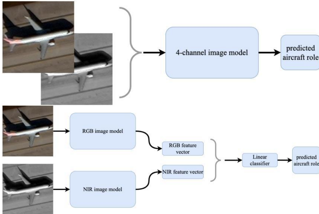
Figure 2: RGB+NIR fusion architectures for classifiers predicting aircraft role. Top: early, bottom: late. Braces denote image/feature concatenation.
