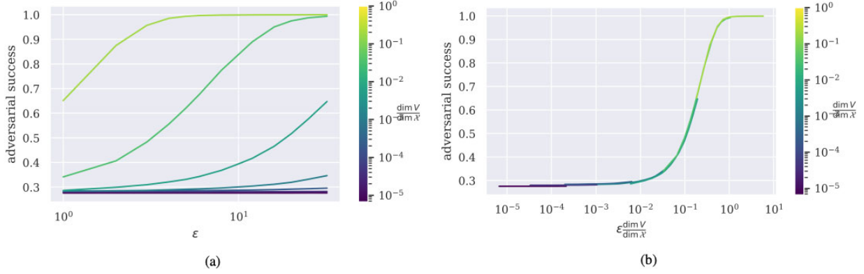
Figure 1: (a) Success of PGD adversarial attacks on an ImageNet trained ResNet50 constrained to subspaces V \subseteq X spanned by \dim V randomly selected standard basis vectors. Adversarial examples are computed for a random subsample of 10,000 datapoints from the ImageNet validations set. The x-axis is the bound \epsilon used during example generation and the different colored curves indicate the dimension \dim V of the subspace to which the examples were constrained to, relative to the dimension \dim X (= 3 \cdot 224^2) of the ambient input space. When only a small number of dimensions can be perturbed, adversarial examples are challenging to generate even with large \epsilon -bounds. (b) These curves become almost perfectly aligned when we reparameterize the x-axis by scaling by \dim(V)/\dim(X) .
