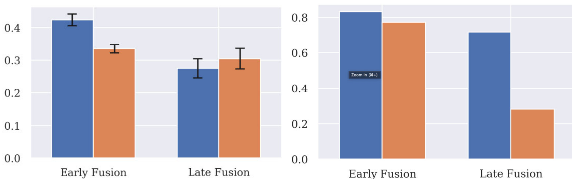
Figure 3: Left: perceptual scores for the multispectral classifiers on the RarePlanes dataset [5]. Blue: RGB, orange: NIR. The early fusion models have a higher perceptual score for RGB channels (i.e., more reliance on RGB inputs), whereas the late fusion models have higher perceptual score for NIR channels (i.e., more reliance on NIR input). Right: perceptual scores for the multispectral segmentation models on the US3D dataset [6]. Both early and late fusion models have higher perceptual scores for RGB data, demonstrating that model performance
