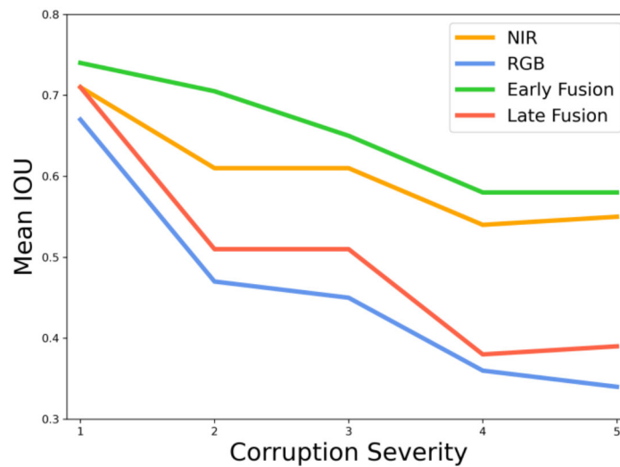
Figure 8: Natural Robustness. Segmentation model performance on data corrupted with physically realistic snow at varying levels of severity (see example datapoints in Figure 7).
