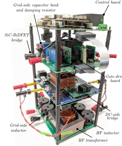
Fig. 6: Hardware prototype of the 2.3 kW, 400 V to 277 V RMS AC/DC DAB converter based on monolithic SiC-BiDFET.
