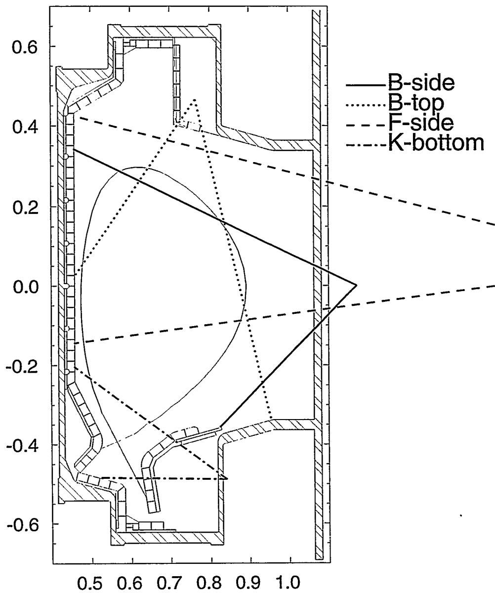
Fig. 2-9: Field of view of the photo-diode imaging arrays. The photo-diode signal, when inverted with a tomographic reconstruction algorithm yields a measurement of a local H_{\alpha} (or Carbon II/IV) emissivity everywhere in the plasma.
