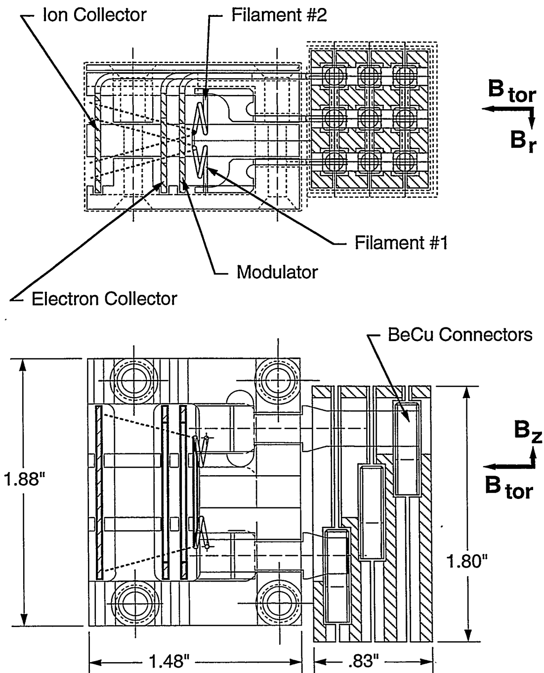
Fig. 3-3: Two views of the gauge and plug assemblies. The drawing also shows the 15° acceptance angles (with respect to the Alcator C-Mod magnetic field components) of electrons emitted from the filament. The nominal dimensions of the assembly elements are also indicated.
