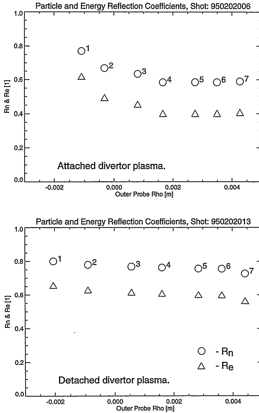
Fig. 5-4: Particle ( R_n ) and energy ( R_e ) reflection coefficients, calculated at each of the outer vertical-target probes, plotted as a function of the probe \rho -coordinate. The top graph shows an example of a hot-attached divertor plasma, the bottom, an example of a cold-detached divertor plasma.
