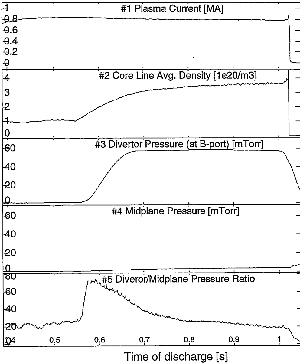
Fig. 1-1: Time history of a high plasma-density Alcator C-Mod discharge. A strong deuterium gas injection between t=0.55 - 0.7 sec causes the core plasma density (trace #2) to increase by about a factor of three but the divertor pressure (trace #3), to increase by about a factor of one hundred. While the 60 mTorr divertor pressure remains constant until the end of the discharge (disruption at t=1.02 sec), the midplane pressure (trace #4) gradually increases, leading to a decreasing divertor-to-midplane pressure ratio (trace #5). This thesis is devoted to experimental study of the phenomena governing the neutral particle dynamics, manifested, e.g., by pressure dependencies shown above.
