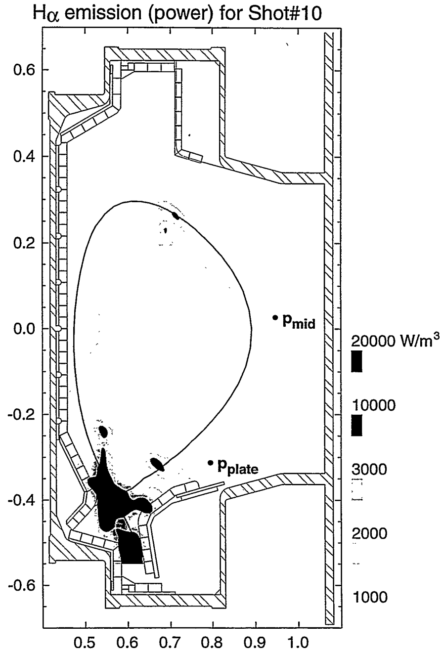
Fig. 5-10: A tomographic reconstruction of H_\alpha emission shows strong poloidal variations indicating neutral density gradients. The neutral pressure near the outer edge of the horizontal target plate ( p_{plate} ) may locally be higher than that measured at the midplane ( p_{mid} ).
