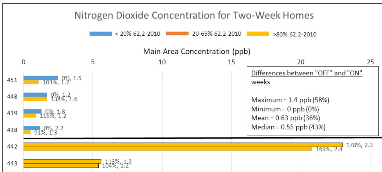
Figure 26. Main area nitrogen dioxide concentrations for two-week homes with at least one gas appliance Data labels indicate the WHMV system flow as a percent of ASHRAE 62.2-2010, and weekly average outdoor nitrogen dioxide concentration.
