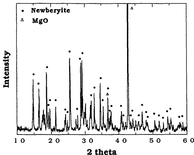
Fig. 1. XRD Pattern of Mono- lithic Magnesium Phos- phate Ceramic.
