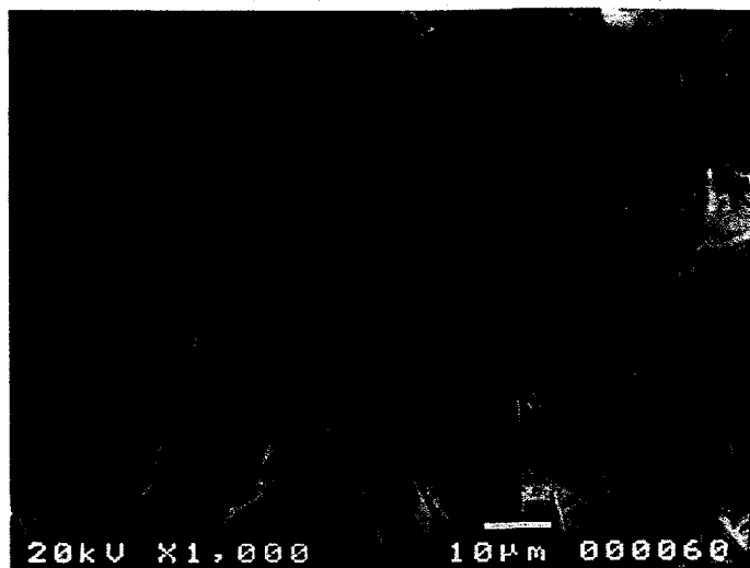
Fig. 2. SEM Photomicrograph of Fracture Surface of Magnesium Phosphate- 35 wt.% Ash Final Waste Form.
