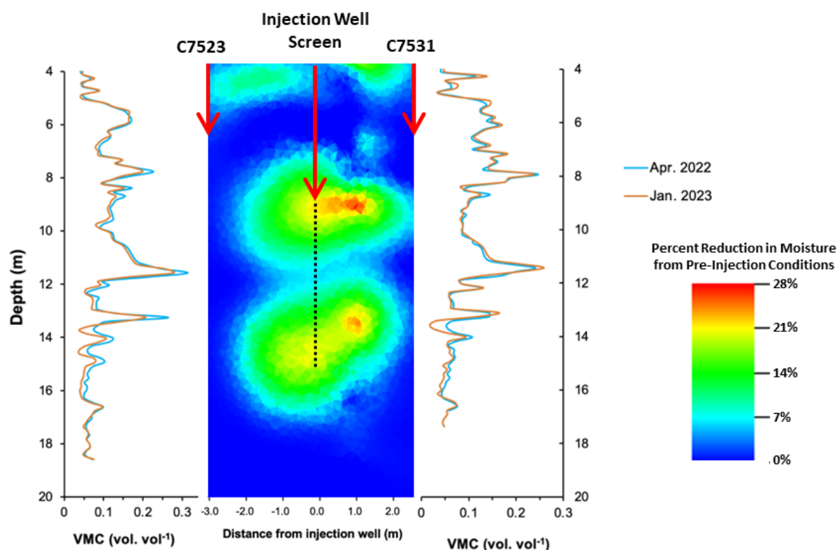
Figure 6. From left to right: Volumetric moisture content (VMC) before and after air injection with depth in logging well C7523 from neutron moisture logging; vertical slice of ERT inversion results between wells C7523 and C7531 showing the percent reduction in moisture from the injection as estimated by the time-lapse ERT data. The screened interval is indicated with a black dashed line; volumetric moisture content from neutron logging, before and after air injection, with depth in logging well C7531 (FIO).
