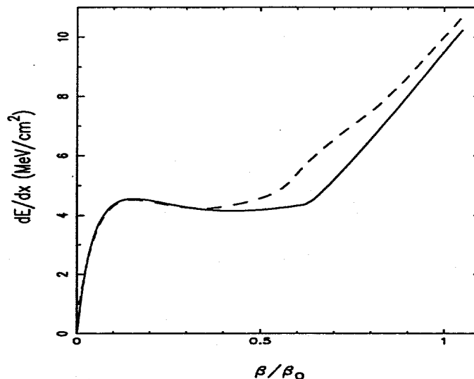
Figure 3: Comparison of total stopping power for ^{151}\text{Dy} ions in Au calculated using TRIM95 (solid line) and by scaling the Northcliffe and Schilling tabulated values (dashed line). The \beta/\beta_0 = 1 value corresponds to the initial recoil velocity of \beta_0 = 0.02266 .
