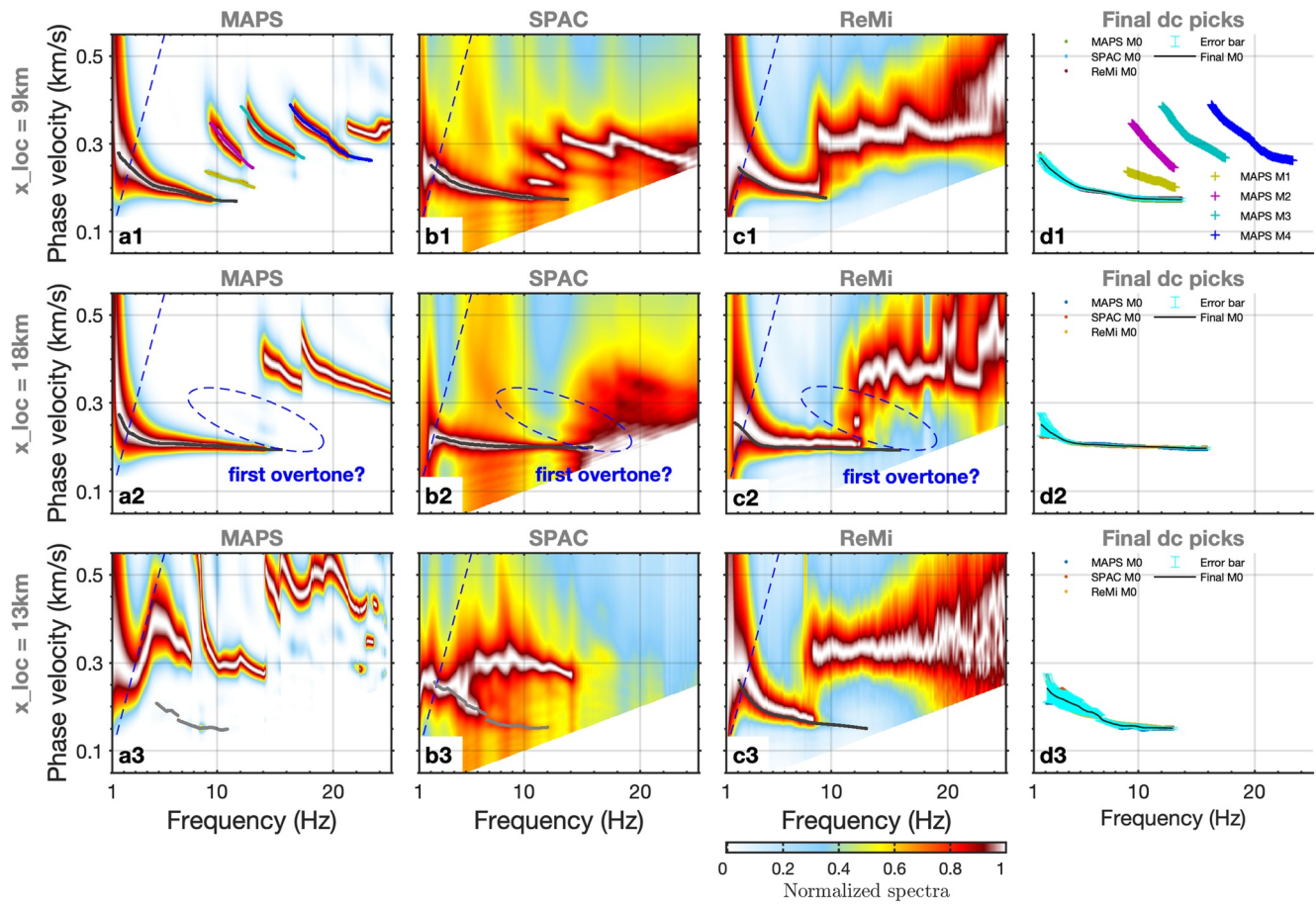
Figure 4. Surface wave dispersion measurements at location 9 km (upper panels), 18 km (middle panels), and 13 km (lower panels) using different techniques, including MAPS (a1, a2, and a3), SPAC (b1, b2, and b3), and ReMi (c1, c2, and c3), and the corresponding picked dispersion curves (d1, d2, and d3). The blue dashed lines indicate the potential maximum resolved wavelength inferred from the profile length. The gray dotted lines that overlay the dispersion spectra indicate the corresponding dispersion picks. The fundamental mode picks from different techniques closely match each other and are overlain with the cyan error bars. The black curves in the right panels show the final smoothed estimated fundamental modes. Note that the fundamental modes on a3 and b3 do exist but appear relatively weak compared with the stronger higher overtones, which are further highlighted by frequency normalized display.
