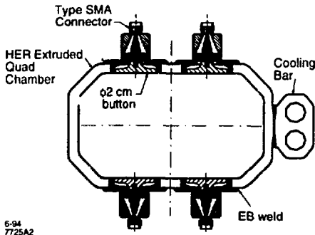
Figure 5 Cross section of quadrupole chamber showing BPM feedthroughs.
