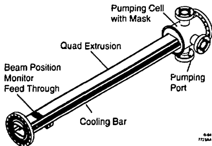
Figure 4 Isometric view of quadrupole vacuum chamber.
