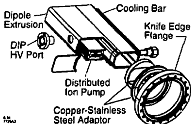
Figure 2 Isometric view of HER dipole vacuum chamber
