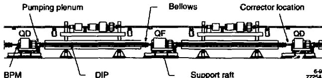
Figure 1. HER arc cell showing dipole and quadrupole chambers
