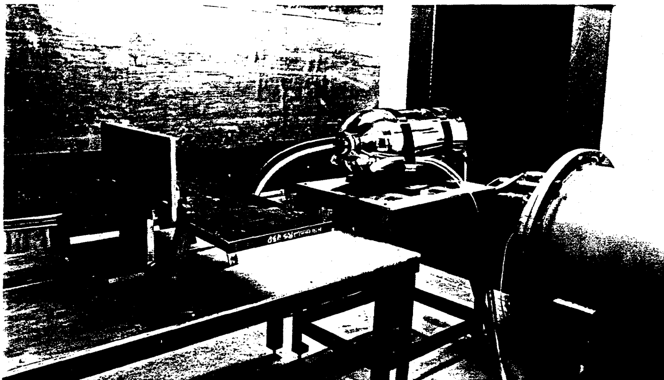
Photograph: Fast neutron radiography system located in the north radiography station cell at Argonne National Laboratory
