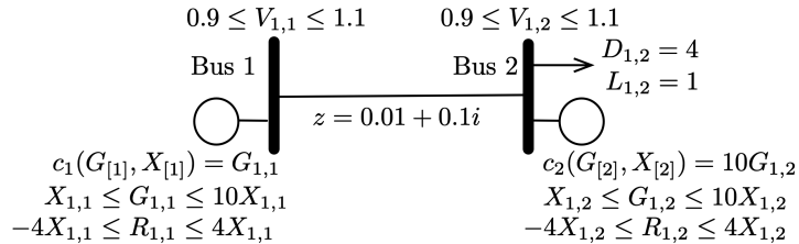
Figure 1: Simple two-bus AC transmission test case.
