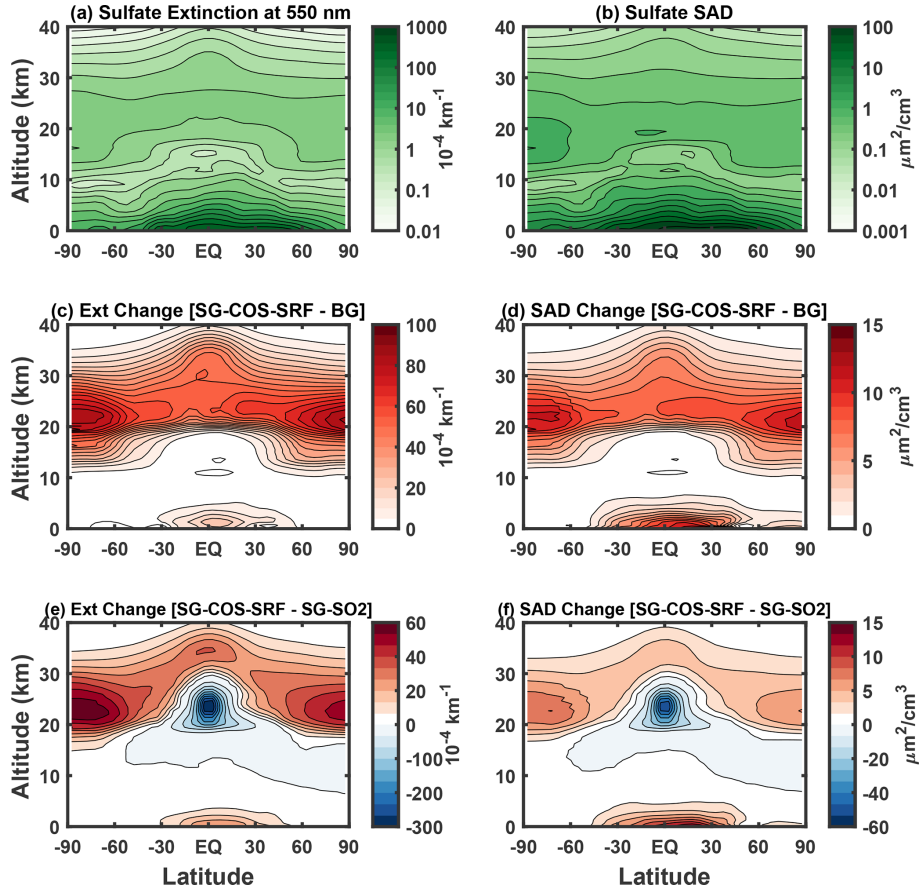
Figure 5. Zonal mean values of sulfate extinction (in 10^{-4} \text{ km}^{-1} ) and SAD (in \mu\text{m}^2 \text{ cm}^{-3} ) in BG (panels a and b , respectively) and their change in the case of the SG-COS-SRF experiment (panels c and d ). Panels (e) and (f) show extinction and SAD changes between SG-COS-SRF and SG-SO2. All quantities are annually averaged over the years 2046–2055.
