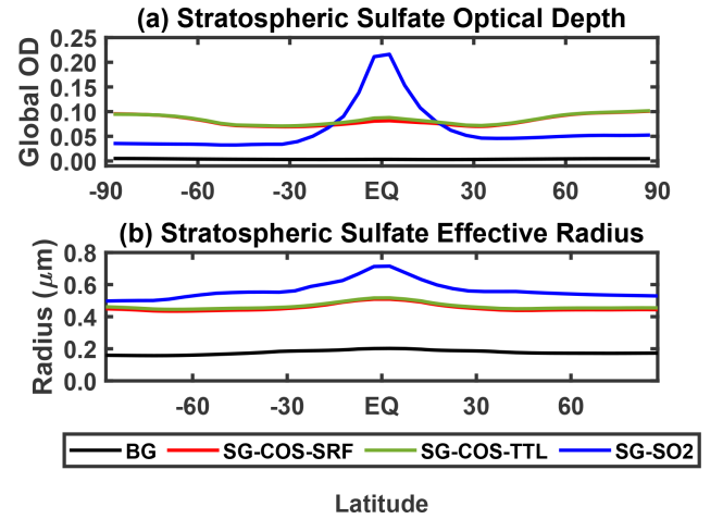
Figure 3. (a) Latitudinal distribution of zonal mean values of the stratospheric sulfate optical depth for the BG (black), SG-COS-SRF (red), SG-COS-TTL (green), and SG-SO 2 (blue) cases. (b) Stratospheric effective radius (in \mu\text{m} , from the tropopause to 6 hPa). All quantities are annually averaged over the years 2046–2055.
