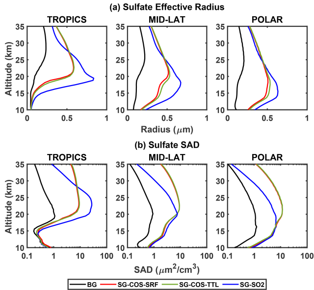
Figure 4. Vertical profiles of sulfate effective radius (in \mu\text{m} ; a ) and surface area density (in \mu\text{m}^2\text{cm}^{-3} ; b ) at different latitudinal bands ( 20^\circ\text{N} – 20^\circ\text{S} for the tropics, 30 – 50^\circ at both N and S for the mid-latitudes, and 60 – 90^\circ at both N and S for the polar plots). All quantities are annually averaged over the years 2046–2055.
