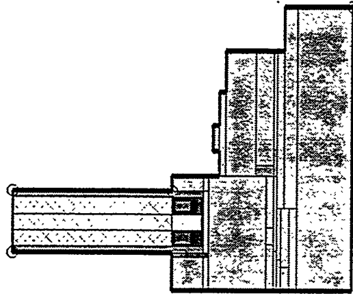
Configuration for the R12.5 super glazing mounted in a wood casement frame. Spacer is steel with a polystyrene foam thermal break. The configuration for the R8 superglazing is similar except that there is only one suspended low-E film.
