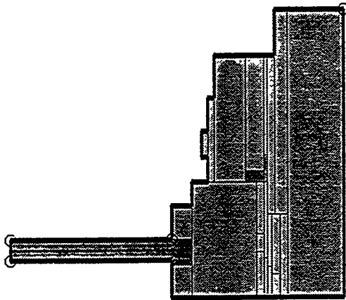
Vacuum glazing mounted in a wood casement frame.
