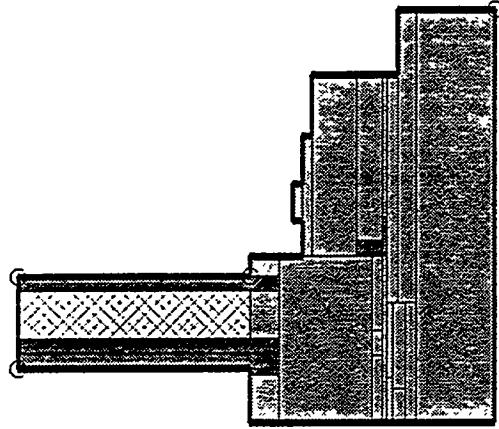
Vacuum glazing with an additional low-E third pane mounted in a wood casement frame. A 12.7 mm.-thick wood spacer reduces thermal bridging through the evacuated glazing edge seal.
