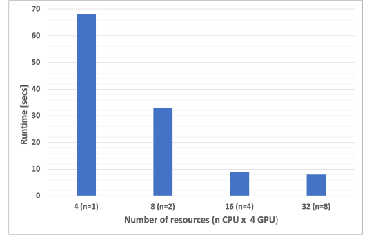
Fig. 5. QASMBench [22] with NWQ-Sim on OLCF Summit computers. Fig. 5 shows QASM benchmark result for NWQ-Sim simulator on the Summit supercomputer. We perform all simulations on the Frontier [19] and Summit supercomputer at ORNL [20] and the Perlmutter supercomputer at NERSC [21].
