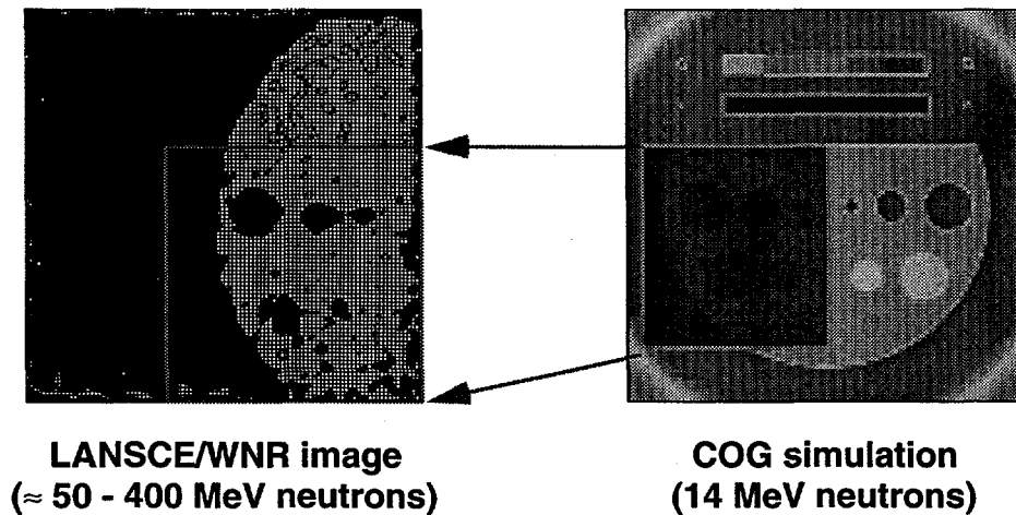
Figure 3: This figure shows the experimental image of the LANSCE/WNR phantom target taken using \approx 50 - 400 MeV neutrons compared to the COG Monte Carlo simulation of a similar phantom for the case of 14 MeV neutrons. Line-outs taken through corresponding regions in the images show similar contrast ratios in the vicinity of the LiD defects in spite of the large difference in incident neutron energies.
