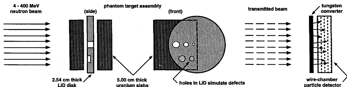
Figure 1: Recent experiments carried out at the LANSCE/WNR facility at LANL have demonstrated the potential for using fast neutron radiography for stockpile stewardship. Neutrons with energies of up to \approx 400 MeV were used to irradiate a uranium and LiD phantom target assembly. Small holes (4 - 12 mm) drilled all or part of the way through the LiD were used to simulate defects. A position sensitive multiwire detector (resolution \approx 1 mm) was used to record the image.
