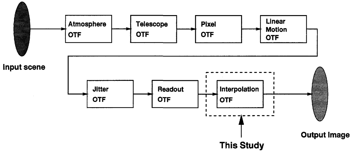
Figure 1: Schematic showing some of the different Optical Transfer Functions (OTF) used in an end-to-end simulation. This study concentrates on the interpolation OTF for registering multispectral digital images.
