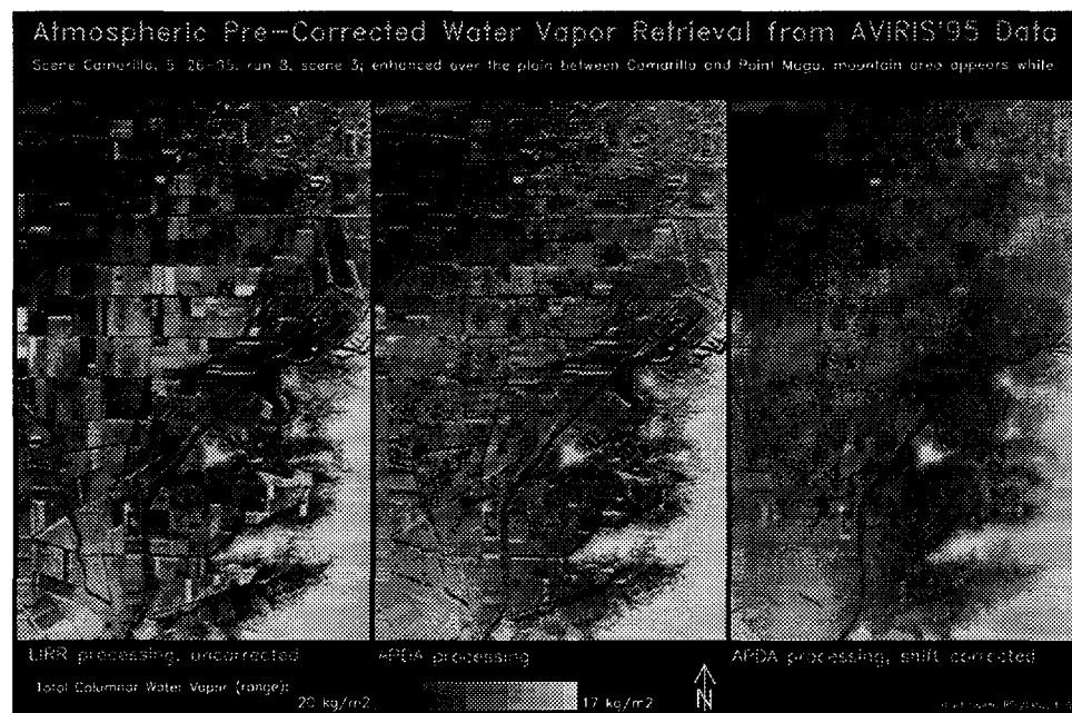
Figure 6: Water vapor retrievals from AVIRIS 1995 images near Oxnard, California, from Schlöpfer et al., (1996). The leftmost panel is the retrieved water vapor map using a technique called the Linear Regression Ratio, or LIRR. The middle panel shows the retrieved water vapor using a technique called Atmospheric Pre-corrected Differential Absorption, or APDA, which corrects for atmospheric path radiance before computing the water vapor. The rightmost panel shows the APDA result with a shift correction applied to the data.
