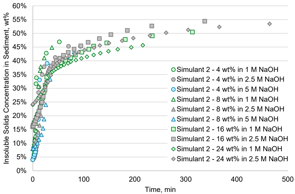
Figure 8 Insoluble Solids Concentration for Simulant 2 (Iron Oxide and Gibbsite)
