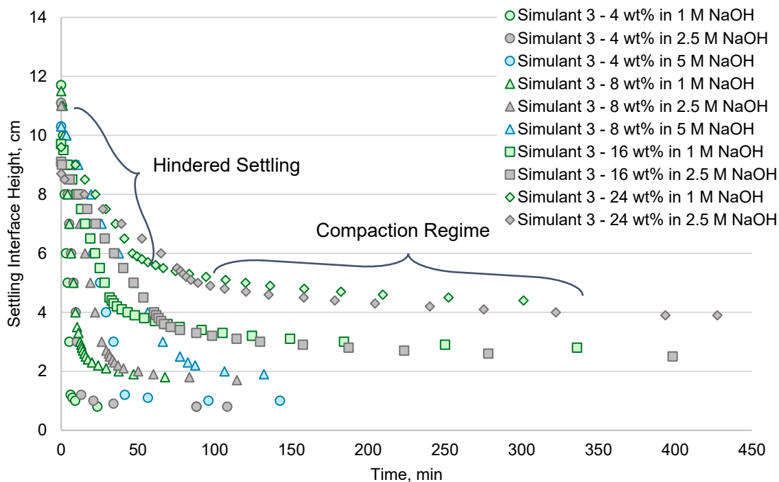
Figure 6 Dimensional Settling Curve for Simulant 3 (Iron Oxide, Boehmite and Gibbsite)
