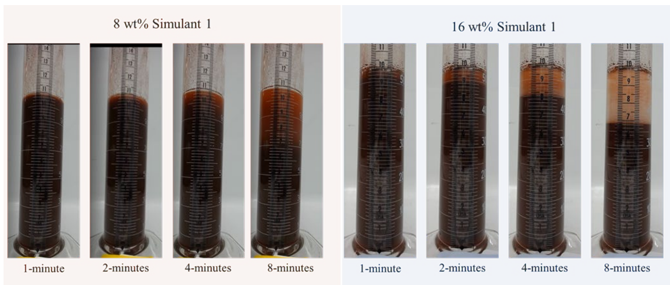
Figure 3 Interface distinction between 8 and 16 wt% at 1-, 2-, 4-, and 8-minute settling intervals
