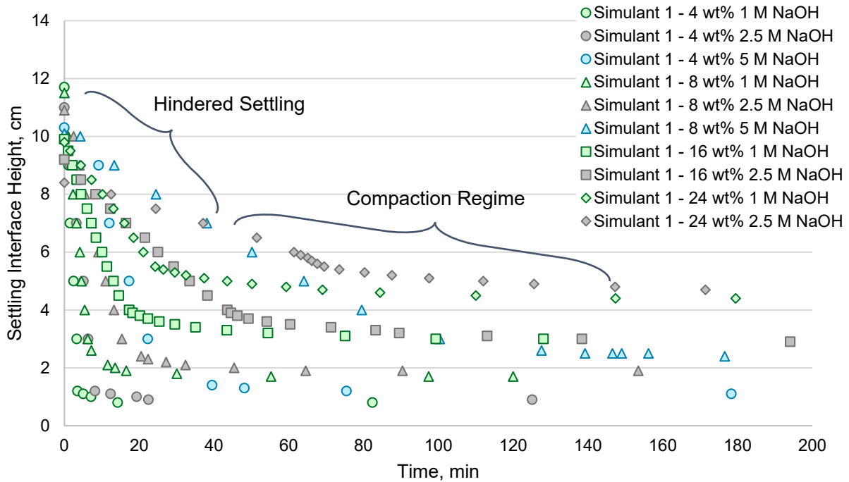
Figure 4 Dimensional Settling Curve for Simulant 1 (Iron Oxide and Boehmite)
