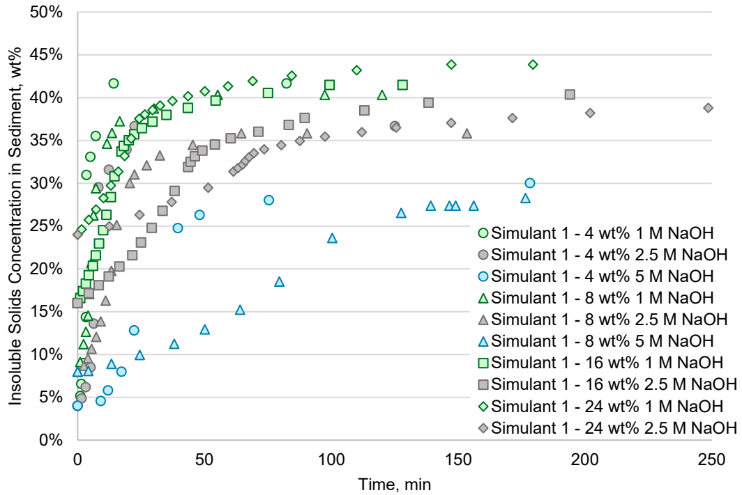
Figure 7 Insoluble Solids Concentration for Simulant 1 (Iron Oxide and Boehmite)
