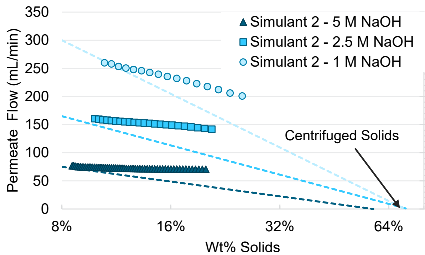
Figure 12 Dewatering of Simulant 2 from 8 wt% to 20 wt% in 1, 2.5 and 5 M NaOH including cake-formation linear flow dependence regime
