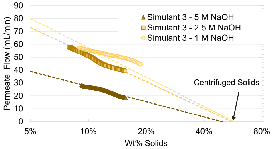
Figure 13 Dewatering of Simulant 3 from 8 wt% to 20 wt% in 1, 2.5 and 5 M NaOH including cake-formation linear flow dependence regime
