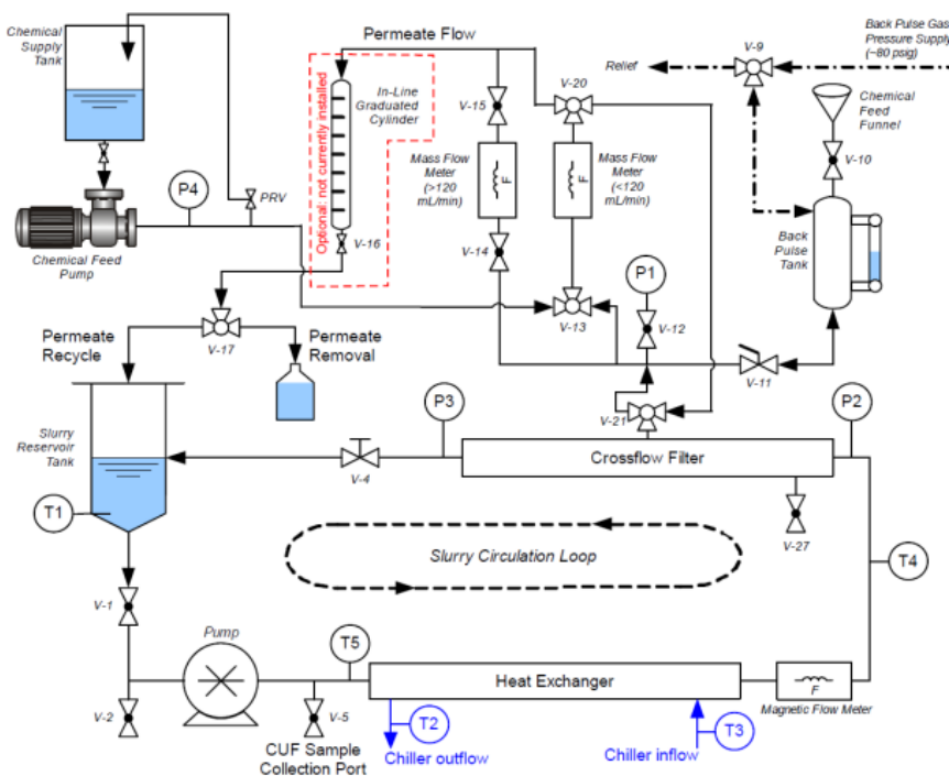
Figure 2 Filter System Piping & Instrumentation Diagram
