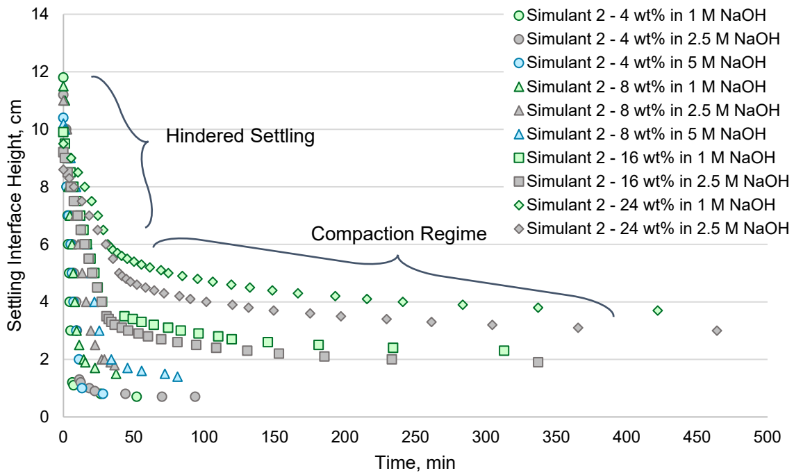
Figure 5 Dimensional Settling Curve for Simulant 2 (Iron Oxide and Gibbsite)
