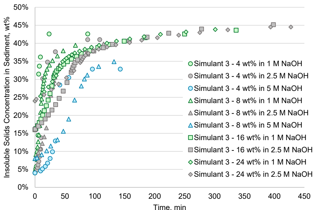
Figure 9 Insoluble Solids Concentration for Simulant 3 (Iron Oxide, Boehmite and Gibbsite)
