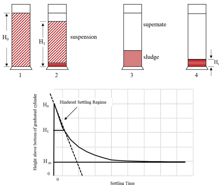
Figure 1 Settling Cycle of a Suspension
