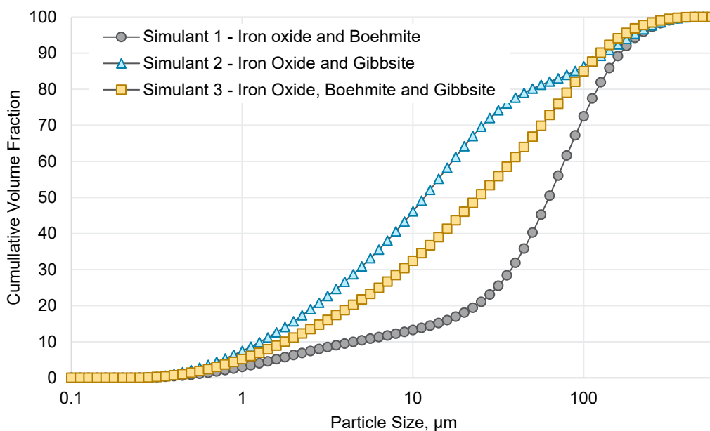
Figure 10 PSD of Slurries on a Volume-Weighted Bases for Simulants 1, 2, and 3 in Cumulative Under-Size-Percentage Distribution
