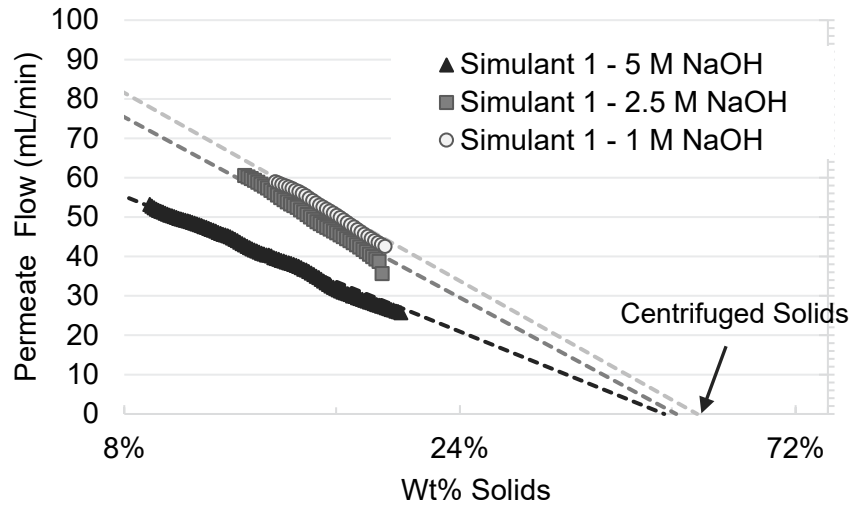
Figure 11 Dewatering of Simulant 1 from 8 wt% to 20 wt% in 1, 2.5 and 5 M NaOH including cake-formation linear flow dependence regime
