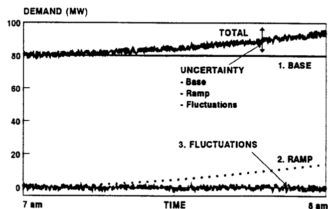
Fig. 1. Components of a hypothetical customer's time-varying load, from 7 am to 8 am on a weekday morning.
