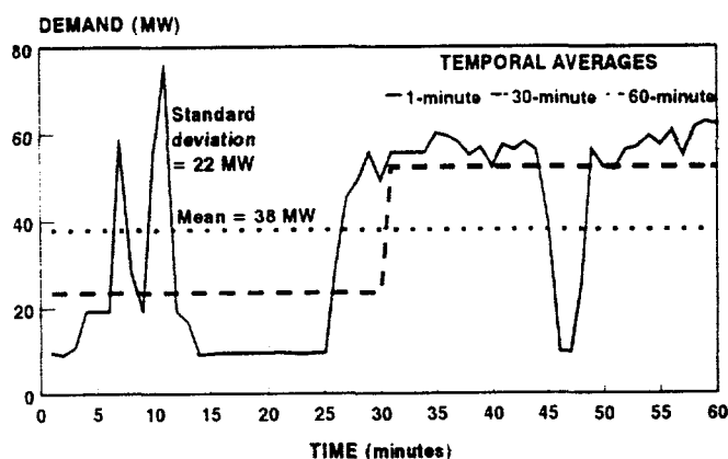
Fig. 2. Minute-by-minute variation in the load of an electric-arc steel mill.
