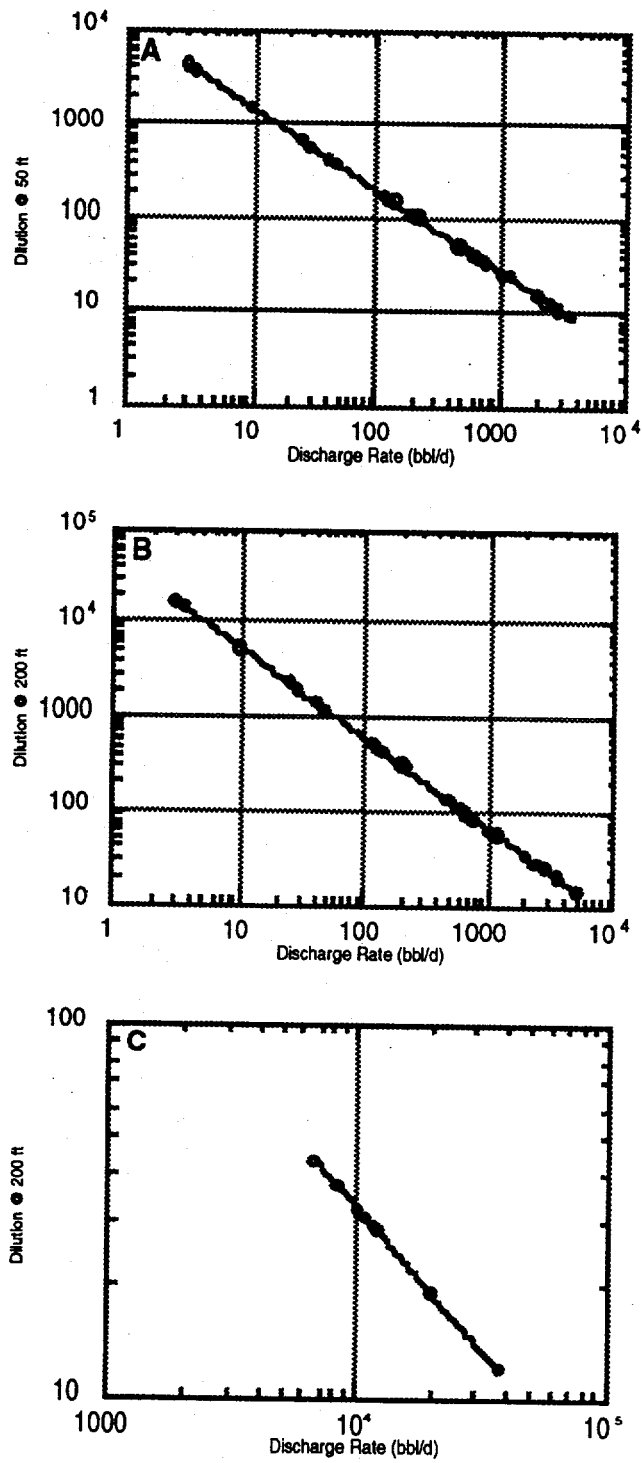
Figure 5-5. Relationships between discharge rates and model-derived dilution factors in the plume at 50 and 200 feet from discharge: A and B, NV2 algorithms; C, NV5 algorithm.
