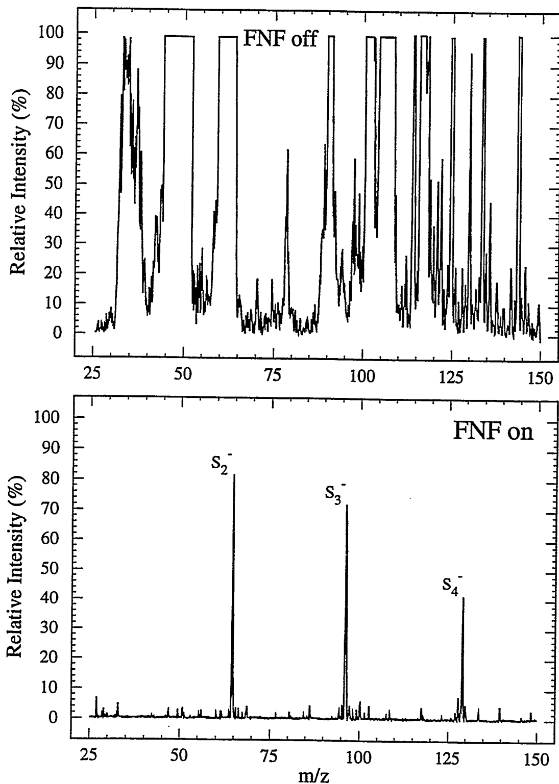
Figure 13. ASGDI mass spectra derived from sampling head space vapors of black powder in the absence of mass selective ion accumulation (a) and using a filtered-noisefield to allow for the selective accumulation of ions at m/z 64, 96, and 128 (b).
