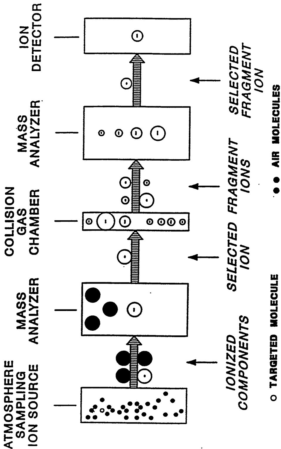
Figure 3. Schematic representation of the ASGDI MS/MS experiment for explosives detection.
