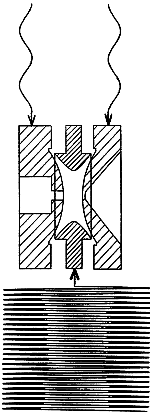
Figure 7. Side-view schematic of the ion trap with a sinusoidal signal applied to the end-caps to effect resonance ejection.
