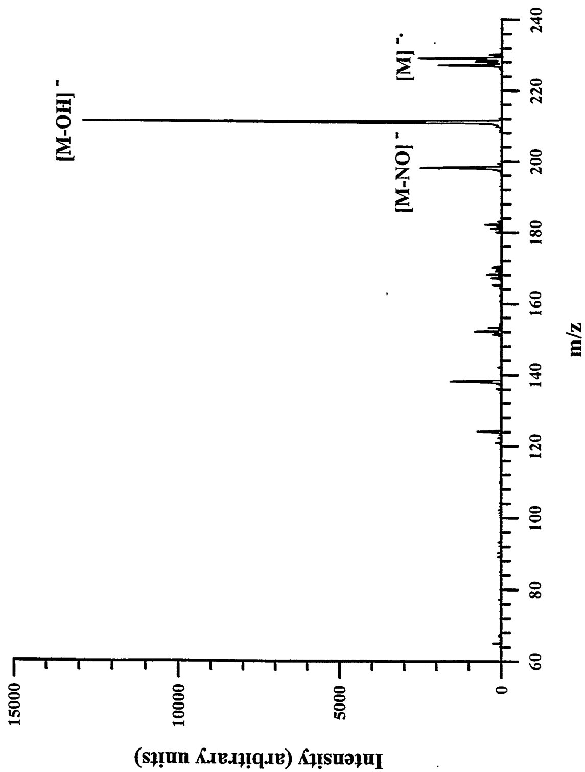
Figure 11. MS/MS spectrum of 2,4,6-trinitrotoluene obtained using single frequency resonance excitation.
