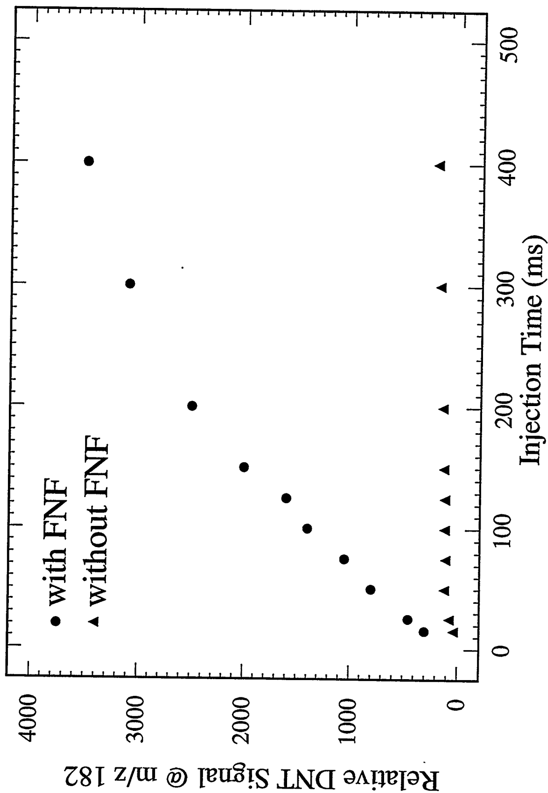
Figure 12. Molecular anions signals of 2,4-dinitrotoluene obtained as a function of ion accumulation time with (filled circles) and without (filled triangles) the use of a filtered-noise field to effect mass selective ion accumulation.
