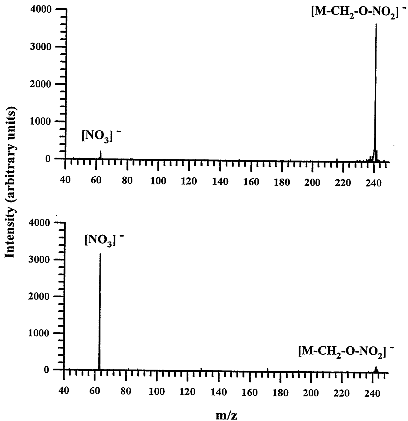
Figure 8. Illustration of the MS/MS efficiency for the (\text{M}-\text{CH}_2\text{ONO}_2)^- anion derived from PETN: (a) spectrum of isolated parent ion (b) spectrum after resonance excitation.
