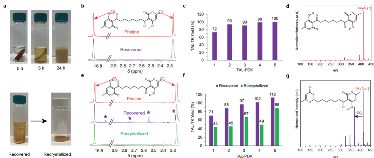
Fig. 2: Recycling of TAL-PDK formulations. a , Acid-catalyzed depolymerization of TAL-PDK 1 plastic and recovery of TAL-TK 1 monomer. b , 1 H NMR spectra of pristine TAL-TK 1 (top) along with crude TAL-TK 1 recovered from chemically-recycled TAL-PDK 1 resin (bottom). c ,
