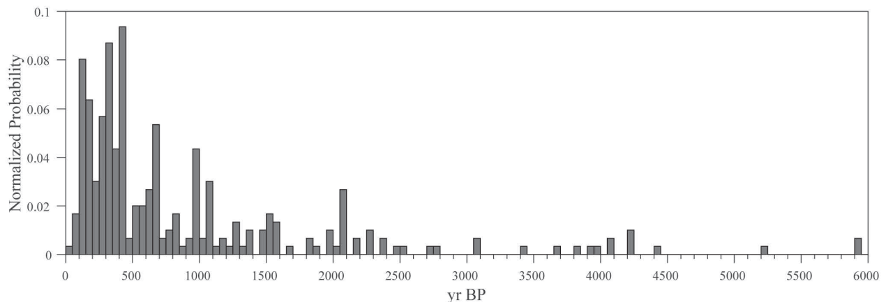
FIGURE 4. Summary of moraine ages in the central Brooks Range based on lichenometry, normalized to total number of moraines sampled (using median age; n = 301 ; 50 yr bins). Ages were calculated using the polynomial fit of Sikorski et al. (2009) and lichen diameters reported by Calkin (1988), Sikorski et al. (2009), Badding et al. (2013), and this study.
