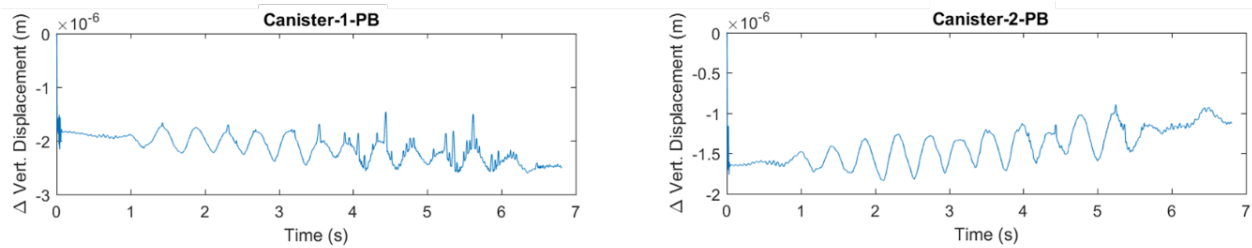
Figure 21. Difference in cask and canister vertical deflection for the 65 mph pitch and bounce test.
