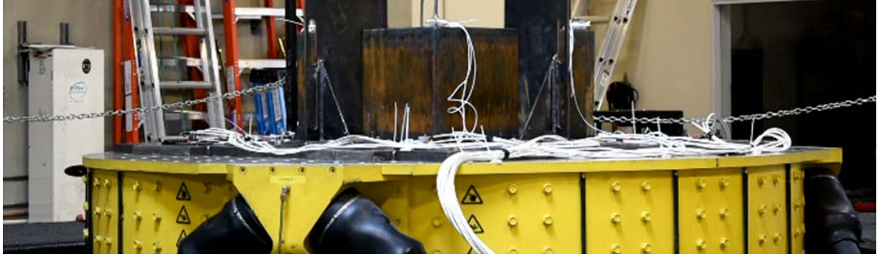
Figure 3. Shaker testing setup.
