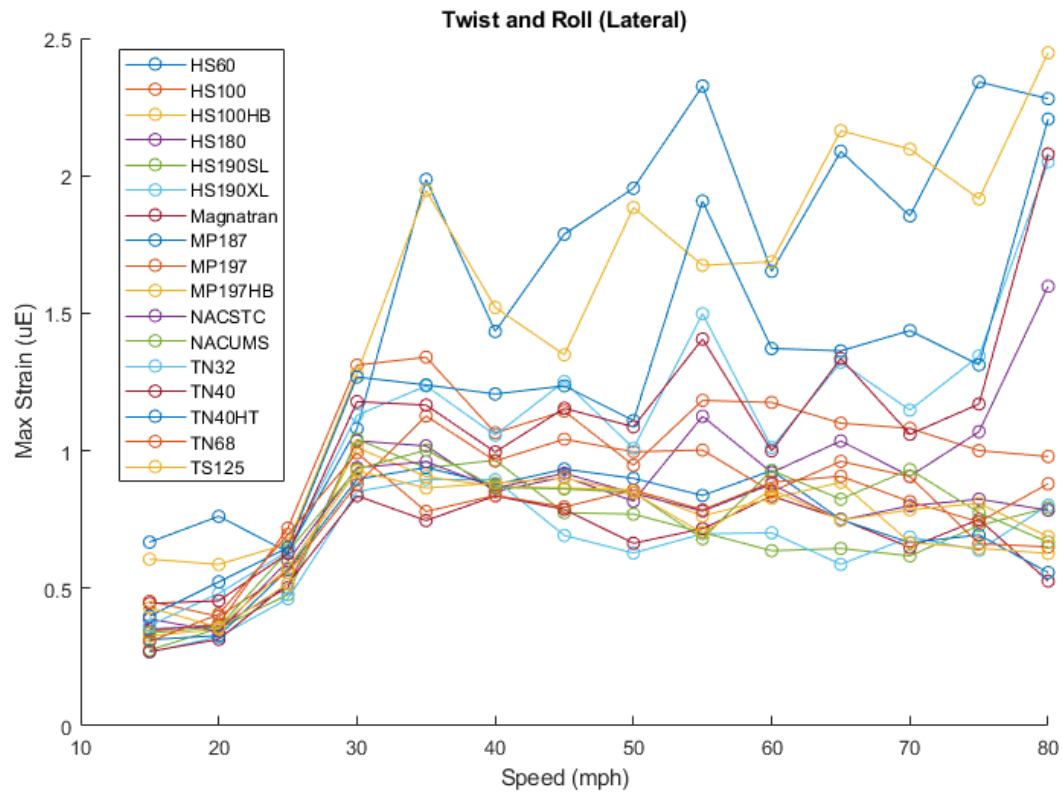
Figure A-10. Peak strain, low-stiffness model on the twist and roll section, lateral loading.
