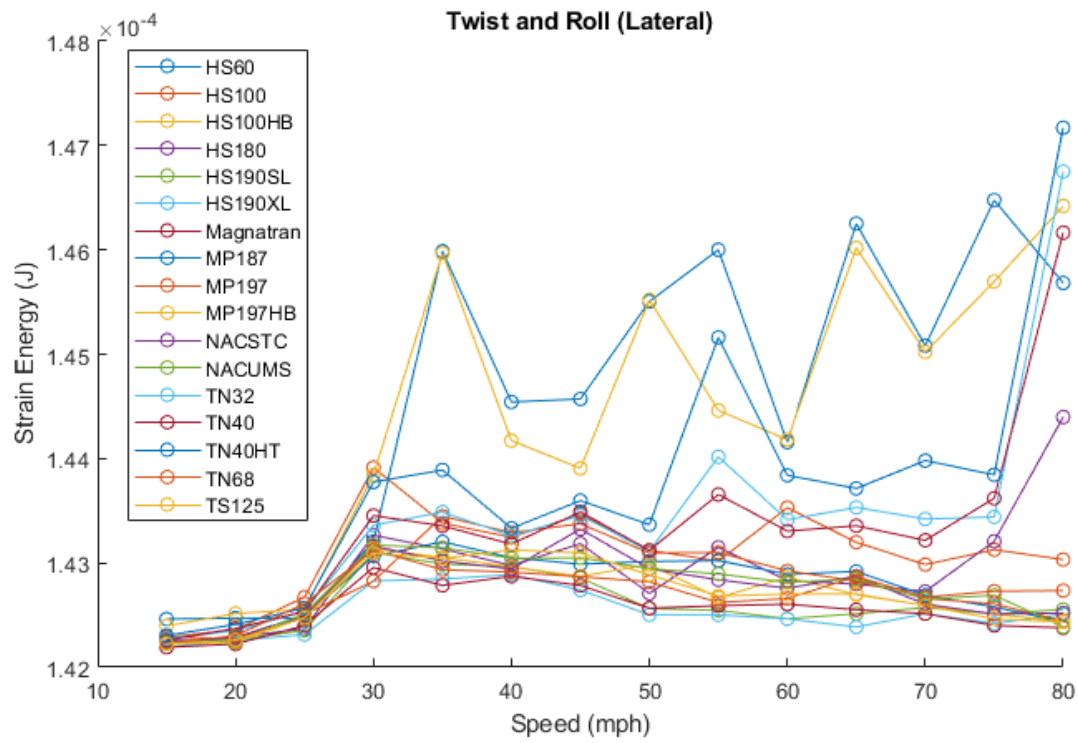
Figure A-23. Peak strain energy, high-stiffness model, twist and roll section, lateral loading.
