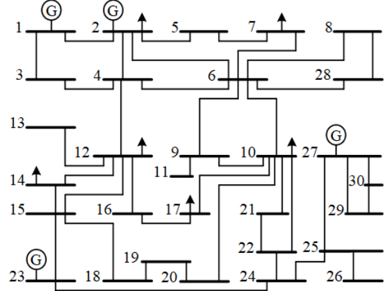
Fig. 6. One-line diagram of IEEE-30 bus system
