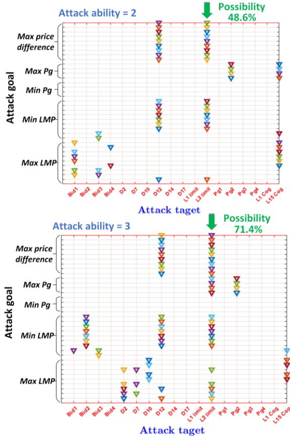
Fig. 7. Identifying the most likely attack target
