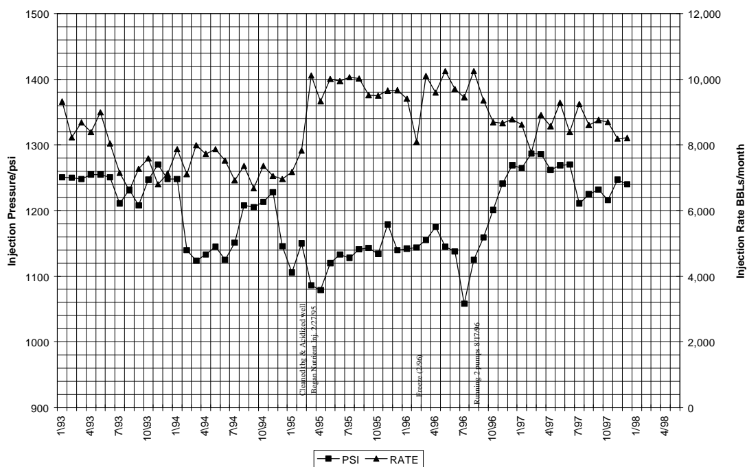
Figure A23. Performance of injection well 34-9 No.2 (test pattern 2).
