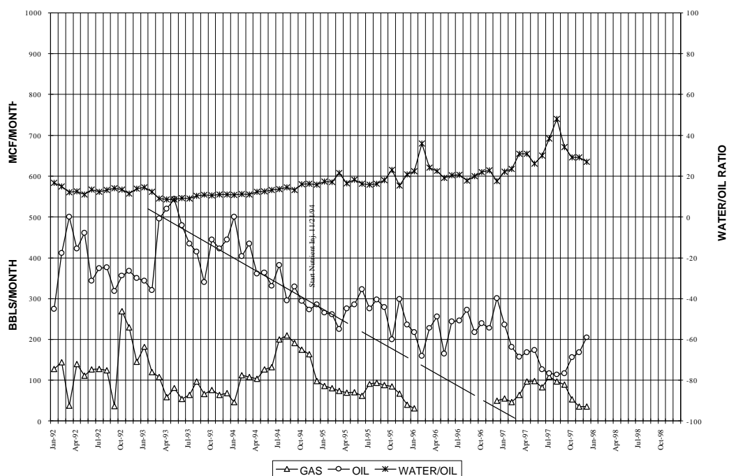
Figure A1. Performance of well 2-11 No.1 (test pattern 1).
