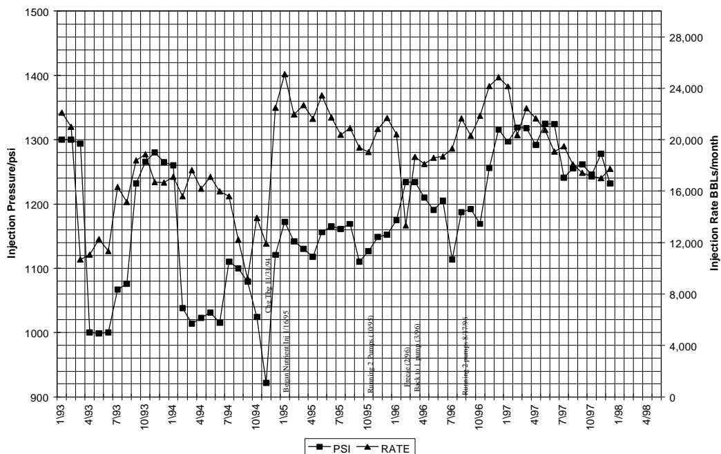
Figure A24. Performance of injection well 11-5 No.1 (test pattern 3).
