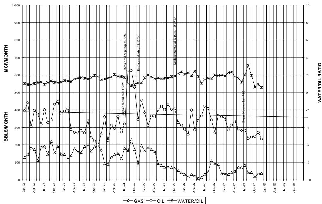
Figure A17. Performance of well 3-1 No.1 (control patterns 1,3,4).
