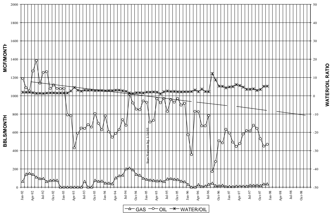
Figure A10. Performance of well 10-8 No.1 (test pattern 3).
