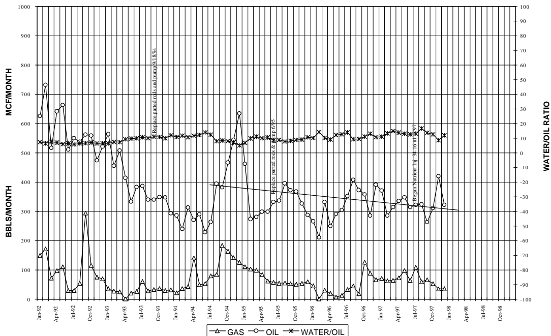
Figure A16. Performance of well 35-13 No.1 (control pattern 1).
