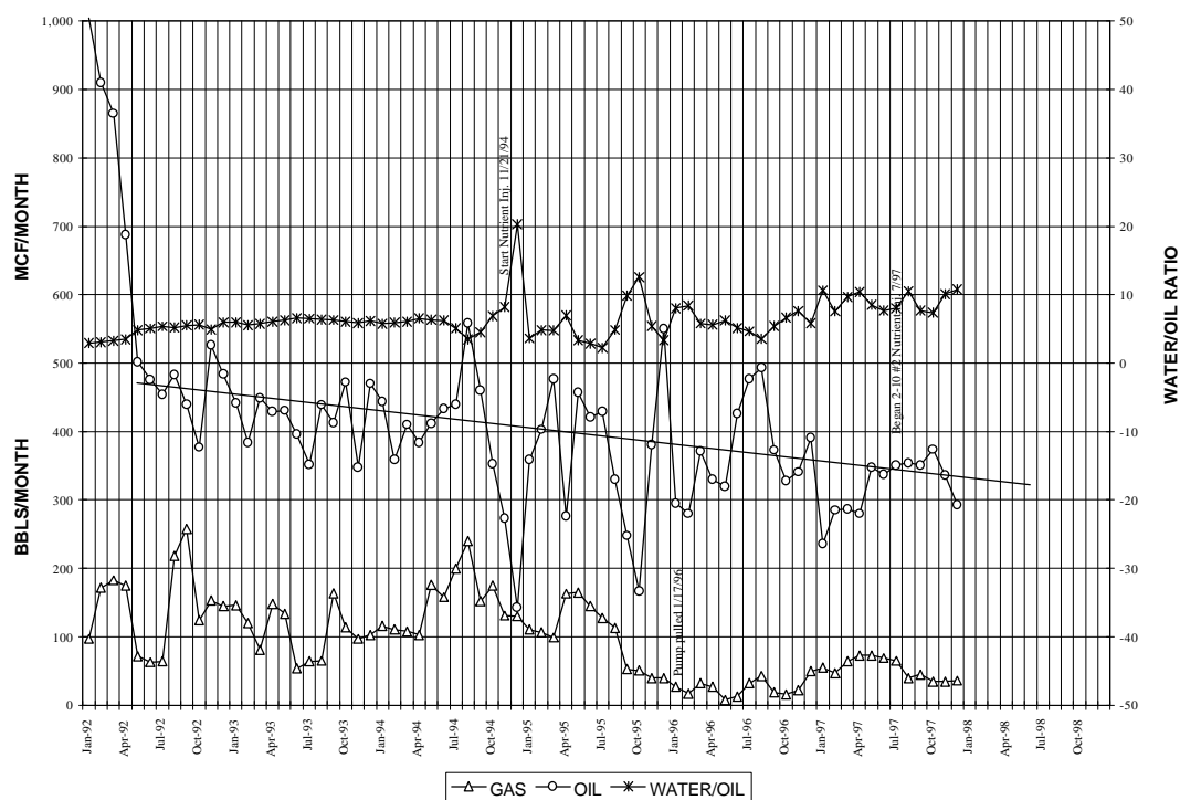
Figure A2. Performance of well 2-15 No.1 (test pattern 1).
