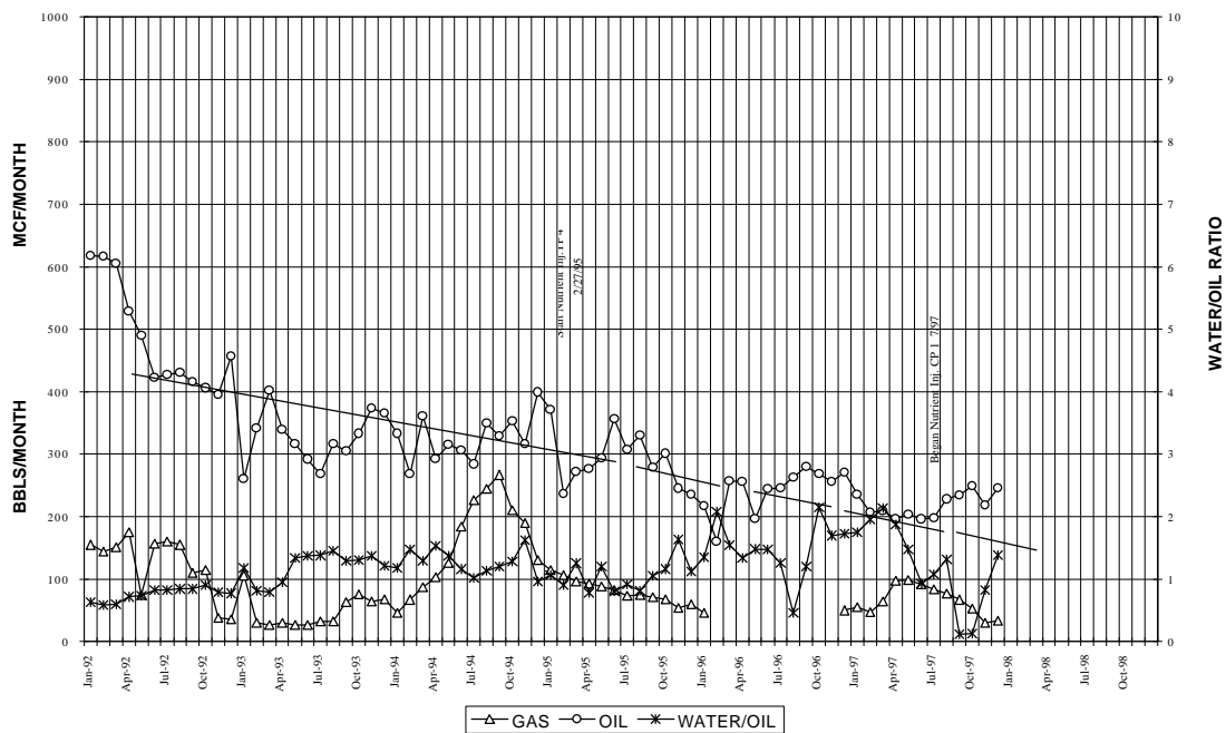
Figure A14. Performance of well 2-3 No.1 (test pattern 4 and control pattern 1).
