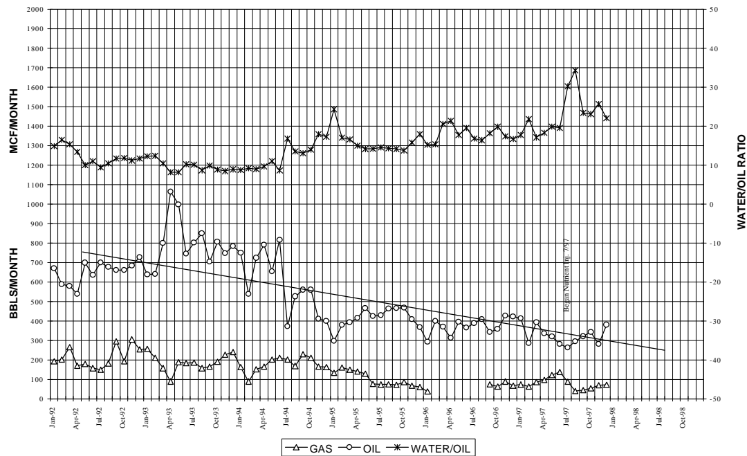
Figure A21. Performance of well 3-9 No.1 (control pattern 4).
