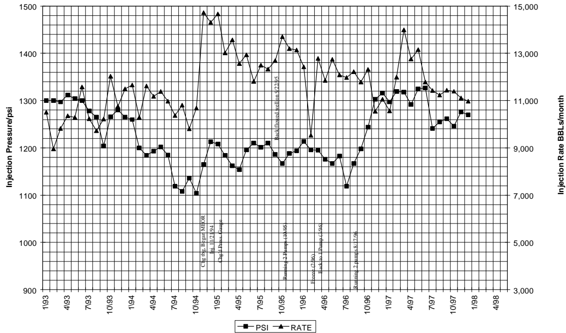
Figure A22. Performance of injection well 2-14 No.1 (test pattern 1).
