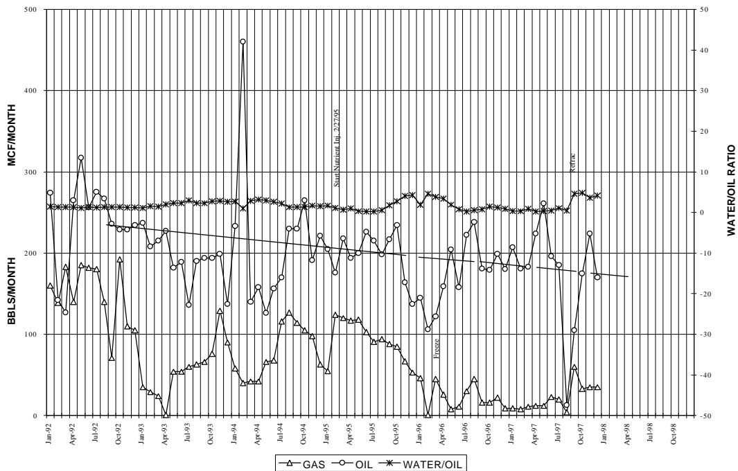
Figure A7. Performance of well 34-15 No.1 (test pattern 2 and control pattern 3).
