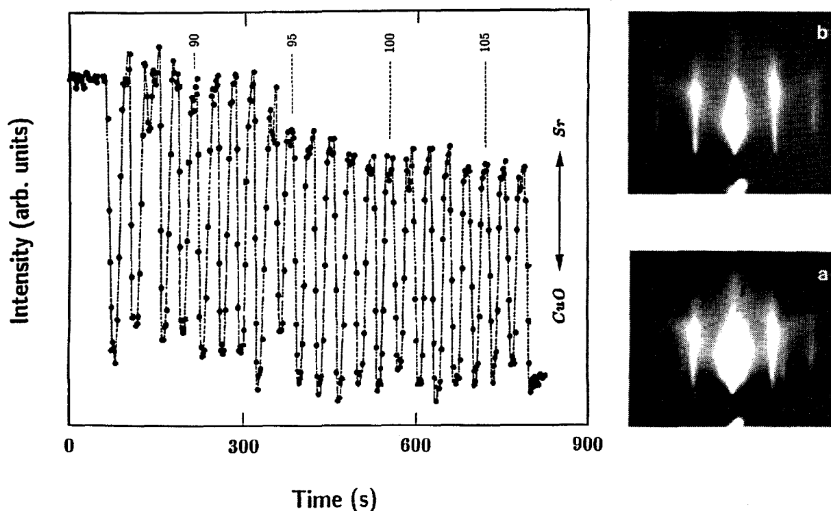
Fig. 2 Intensity variations of the specular reflection in RHEED induced by the alternate deposition of Sr(O) and CuO monolayers during layer-by-layer growth of a \text{Sr}_2\text{CuO}_2 infinite layer film. The intensity increases during Sr(O) deposition and decreases during CuO deposition. Numbers indicate the approximate number of deposited \text{Sr}_2\text{CuO}_2 unit cell layers. RHEED patterns correspond to the minima ("a": after CuO deposition) and maxima ("b": after Sr(O) deposition) of the oscillations, respectively. The electron beam is incident along the [100] azimuth of the substrate at a glancing angle of approximately 1-2^\circ .
