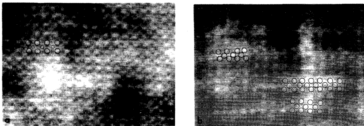
Fig. 3 Cross section Z-contrast STEM images of \text{Sr}_z\text{CuO}_2 infinite layer films grown by ALE: (a) with periodic depositions of \text{Sr}(\text{O}) and \text{CuO} monolayers, and (b) with inserted \text{SrO} defect layers. In (a) Sr and Cu positions have been marked by large and small circles, respectively. Sr positions in extended defects have been marked in (b). Note the formation of triple layers and small lateral dimensions of the \text{SrO} defects.
