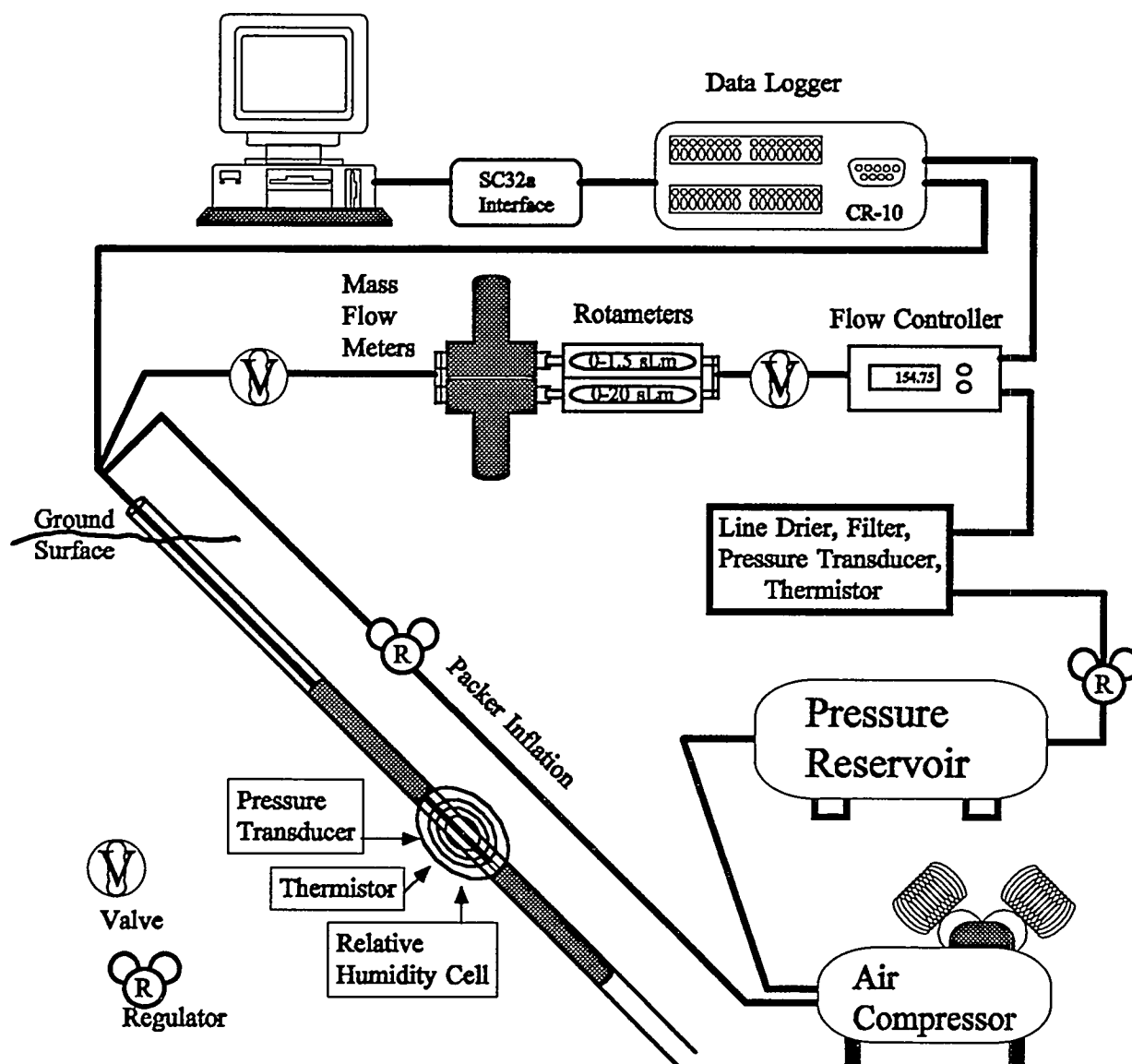
Figure 2.1 Schematic diagram of the air injection system.
