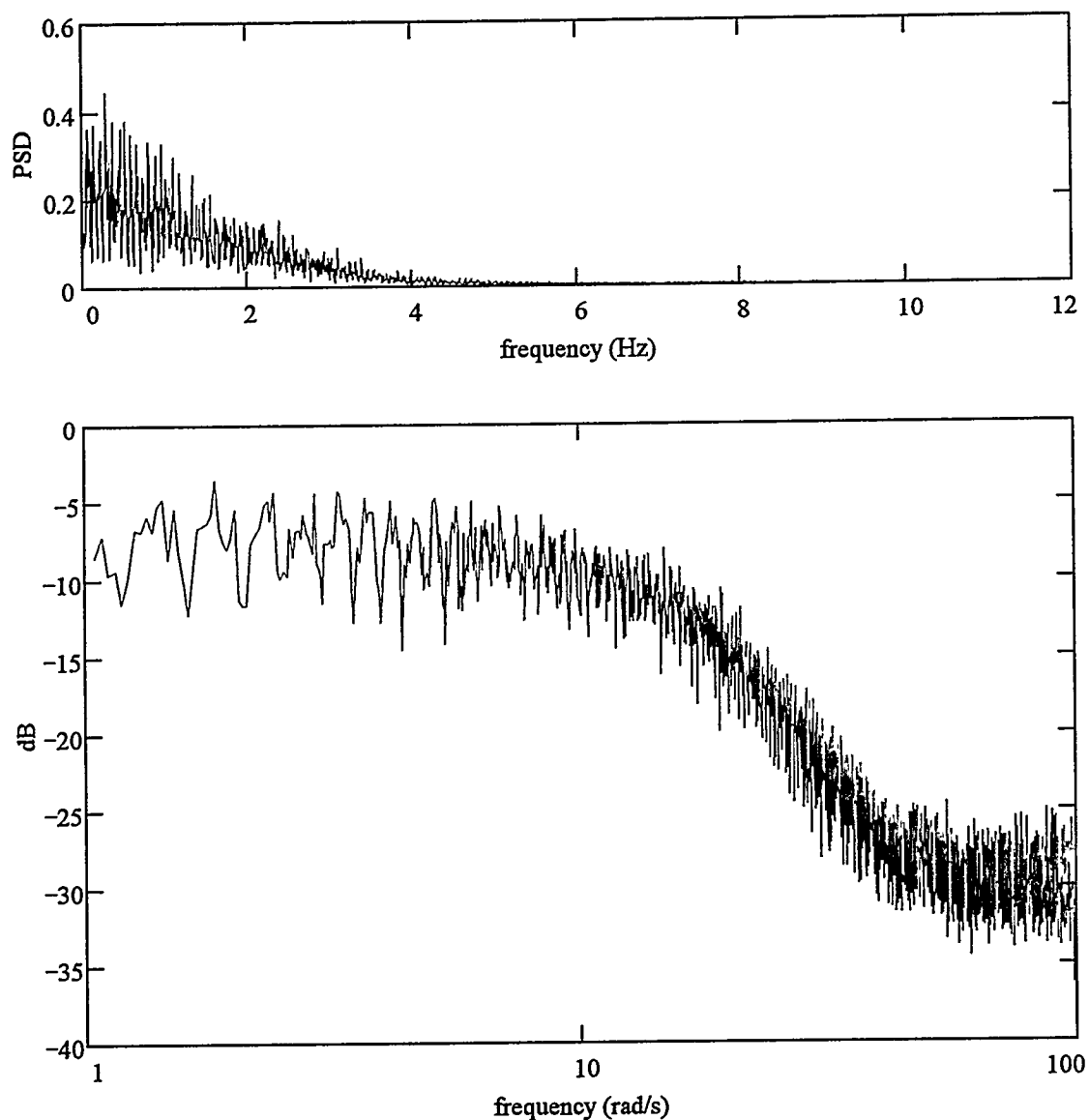
Figure 3: PSD and Bode plot of BFB fluctuations above the bed
