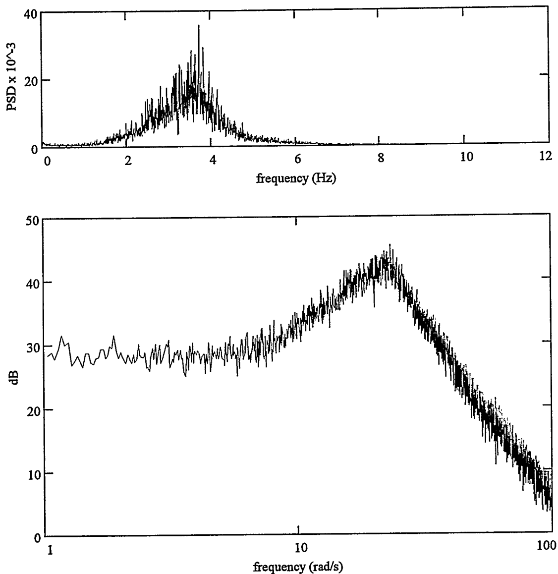
Figure 17: PSD and Bode plot of BFB fluctuations with 36 hole distributor
