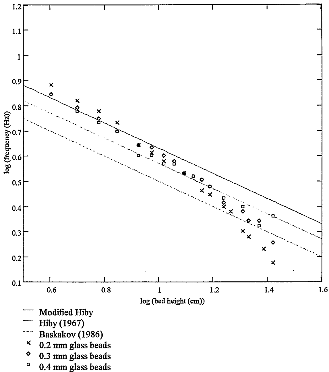
Figure 31: \log - \log comparison of modified Hiby model to experimental data ( D = 4.0'' ) \log(\text{frequency}) vs. \log(\text{only the lowest dominant BFB frequency observed})
