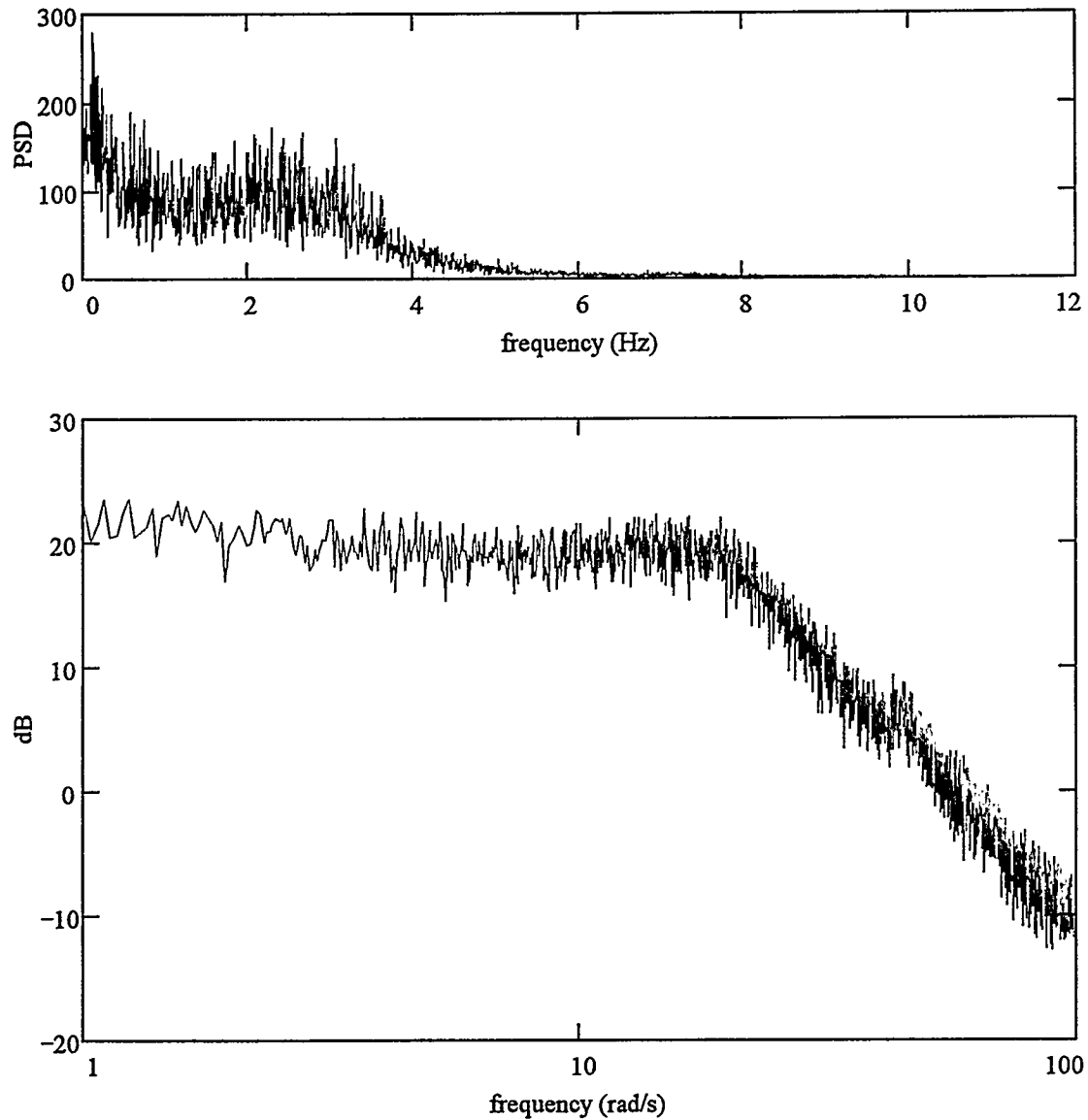
Figure 5: PSD and Bode plot BFB fluctuations with 2.0"(5.1 cm) tap spacing
