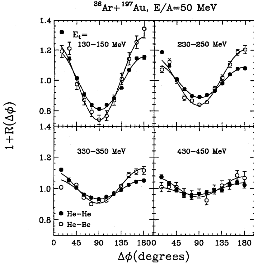
Figure 1. Evolution of the azimuthal correlation functions of two He particles (solid circles) and He and Be particles (open circles) emitted at \theta_{lab} = 31^\circ\text{-}50^\circ for four different cuts on the transverse energy E_t from the reaction ^{36}\text{Ar} + ^{197}\text{Au} at E/A=50 \text{ MeV} . The solid lines are fits of the form given in Eq. (10). The error bars are statistical.
