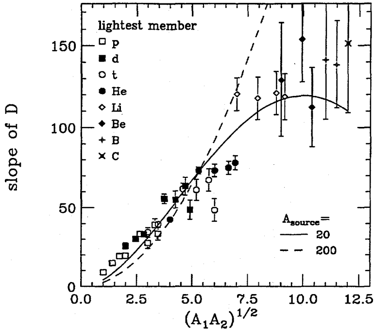
Figure 3. Slope of D (see Fig. 2) as a function of \sqrt{A_1 A_2} for particles with mass numbers between 1 and 12. The most abundant isotope in the periodic table is assumed for the mass numbers of the indicated elements. The lightest member of the particle pair is indicated by the different symbols. The solid (dashed) line is a prediction of the mass scaling assuming emission from a source of size A_{source}=20 (200).
