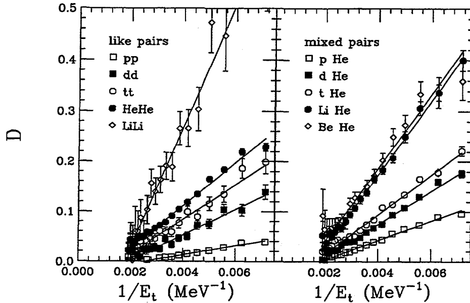
Figure 2. Mass and “temperature” dependence of D . Left panel: The fit parameter D = \lambda_2/(1 - \lambda_2) as a function of 1/E_t (\propto 1/T^2) for the indicated identical particle pairs. Solid lines are linear fits to the data. Right panel: Same as left panel but for particle pairs of different masses.
