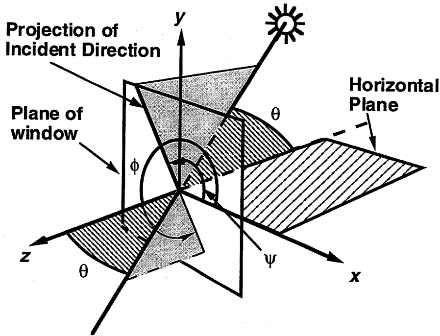
Figure 4. Relation Between Sun Angles ( \theta, \psi ) and Layer Coordinates ( \theta, \phi ).
