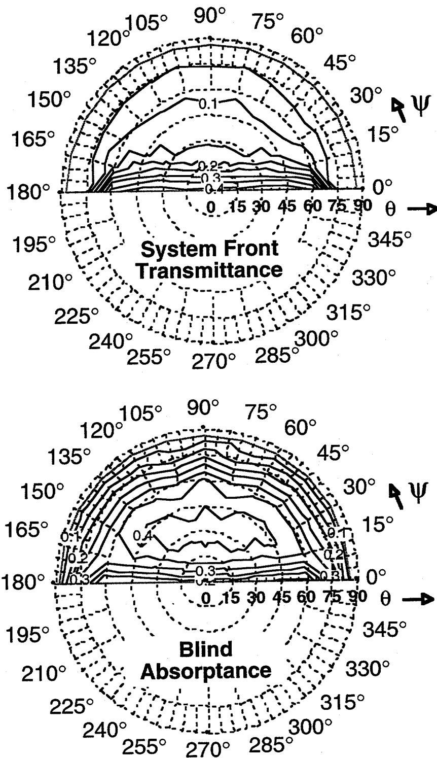
Figure 8. Contour Plots of the Directional System Front Transmittance and Blind Absorptance in the Sky Half-Hemisphere.
