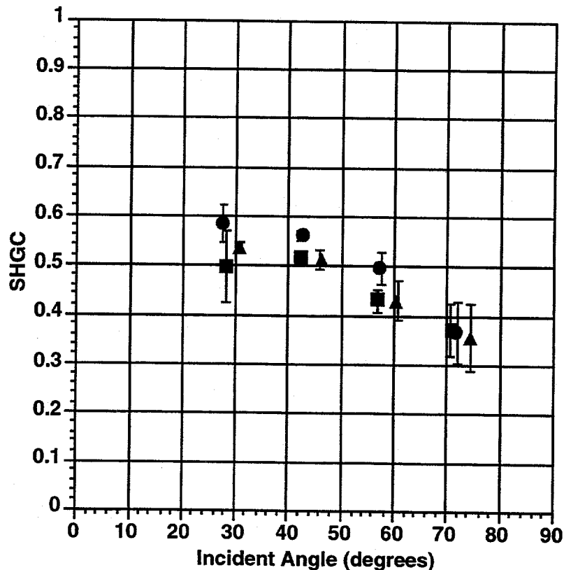
Figure 1. Angle-Dependent Solar Heat Gain Coefficients for the Venetian Blind Derived from MoWiTT Data. Squares: October 1988 measurement period; triangles: August 1989 measurement period; solid circles: September 1991 measurement period.
