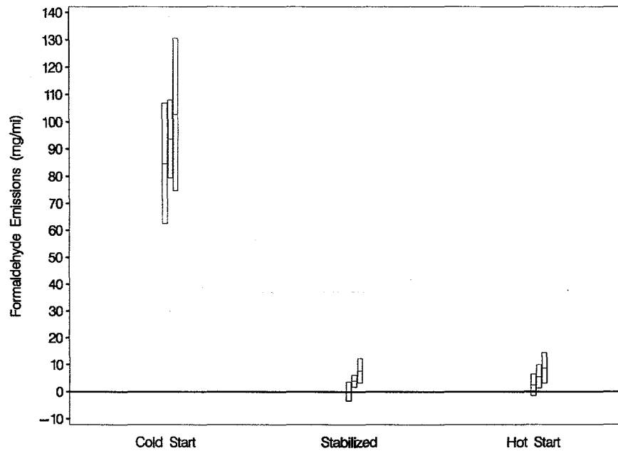
Figure 13. Emission Levels of Formaldehyde from M-85 Vans Measured in the Cold Start, Stabilized, and Hot Start Phases of the Test Procedure (For Each Phase, Mean Emissions are Presented at 5,000, 15,000, and 25,000 Miles, Along with 95 Percent Confidence Intervals)
