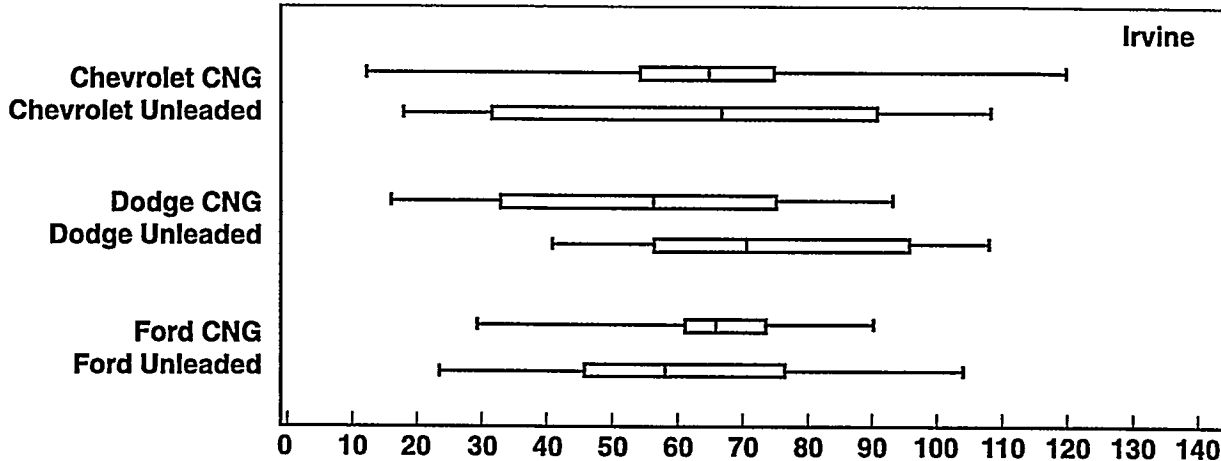
Figure 4. The distribution of the average miles that CNG and control vehicles traveled each day overlaps, providing comparable routes.
