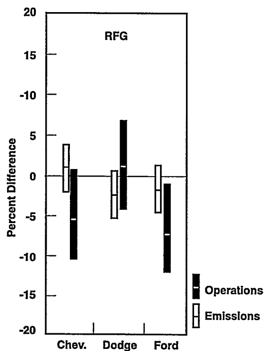
Figure 23. Relative fuel economy (efficiency) for RFG vans was compared to the control vehicles.
