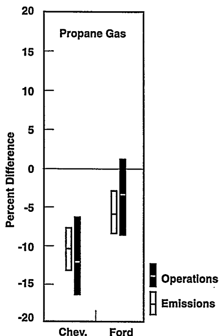
Figure 15. Relative fuel economy (efficiency) for propane gas vans was compared to the control vehicles.
