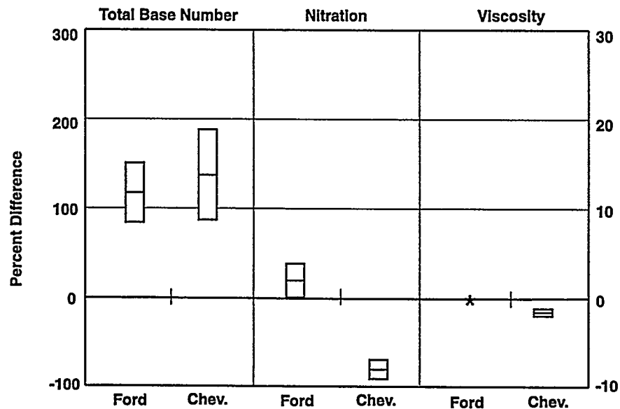
Figure 17. Relative differences in total base number, nitration, and viscosity of used motor oil after 3,000 miles were normalized for propane gas and control vans.
